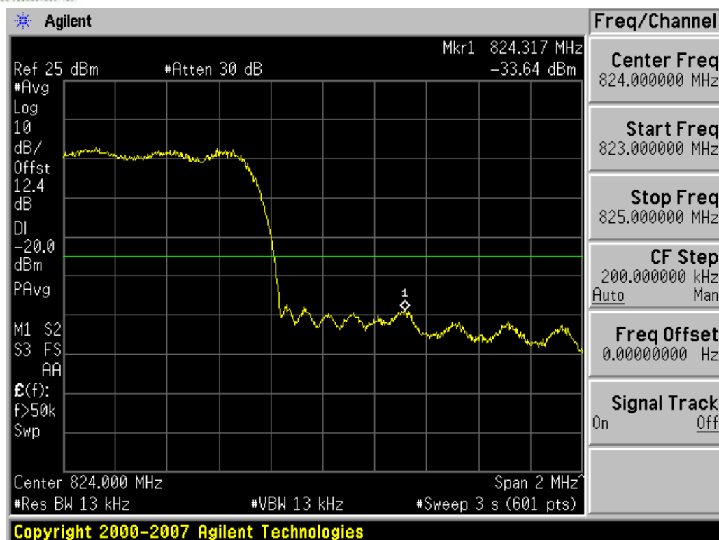
Plot 7-10. Channel Edge Plot (BC10 CDMA Ch. 684) - S90.691
