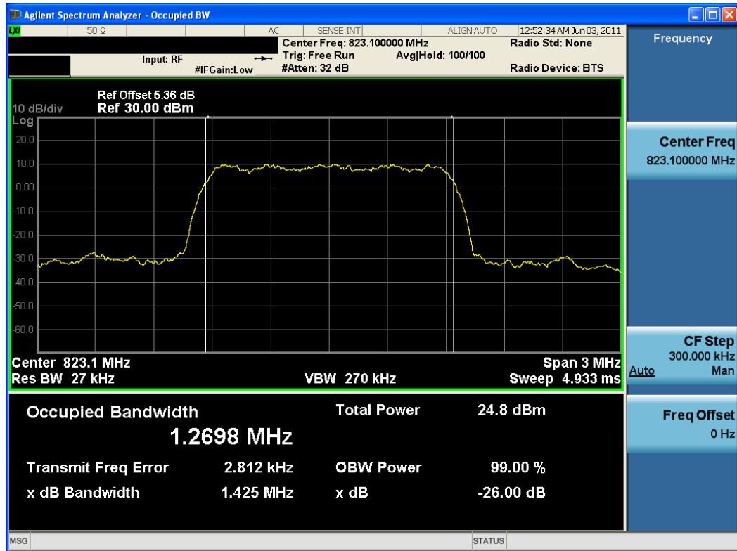
Plot 7-12. Occupied Bandwidth Plot (BC10 CDMA Ch. 684)
