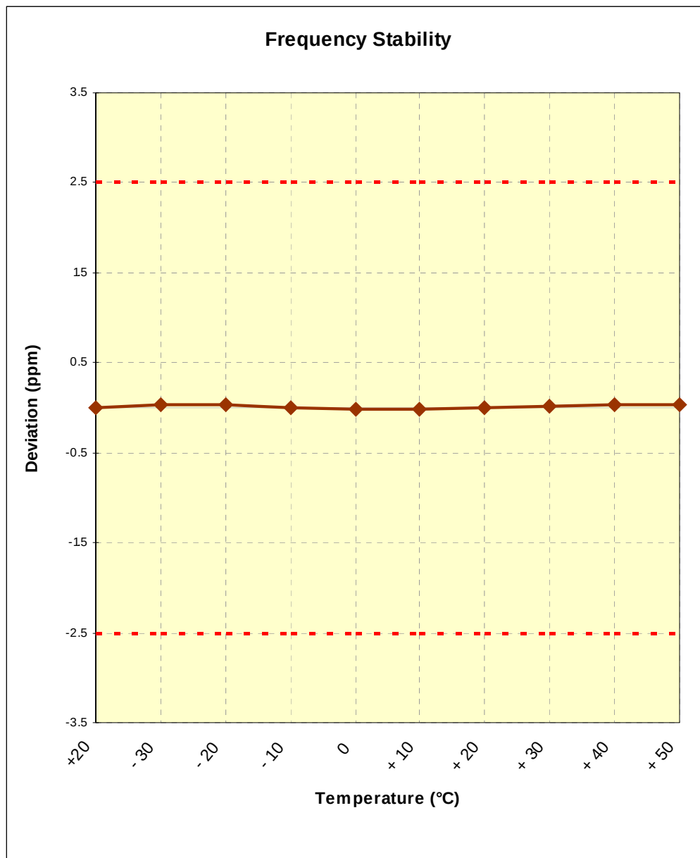
Figure 6-1. Frequency Stability Graph (BC10 CDMA Mode – Ch.684)
