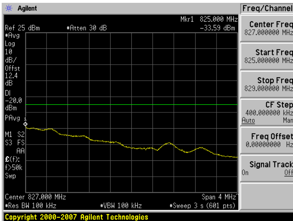
Plot 7-11. 4MHz Span Plot (BC10 CDMA Ch. 684)
