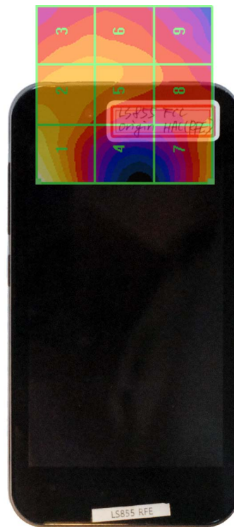
Figure 17-5 H-Field WD Scan overlay
