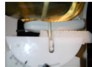
Fig. 14 Head SAR Test Setup
