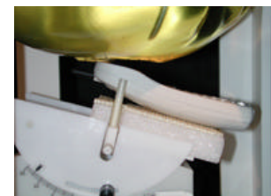
Fig. 12 Head SAR Test Setup
