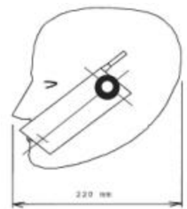
Fig. 10 Cheek/Touch Position
