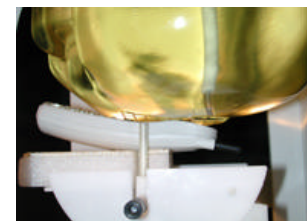
Fig. 15 Head SAR Test Setup
