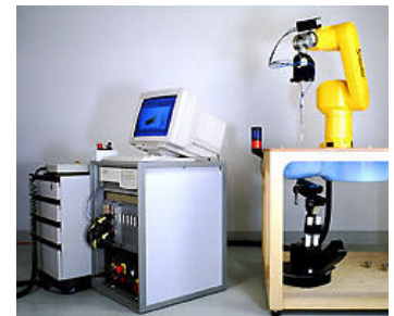
Fig. 1 SAR Test Setup
