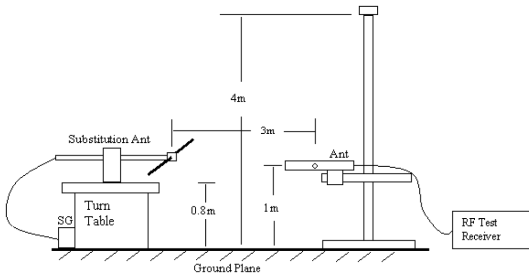
Figure3. Radiated Emission – Substitution Method
