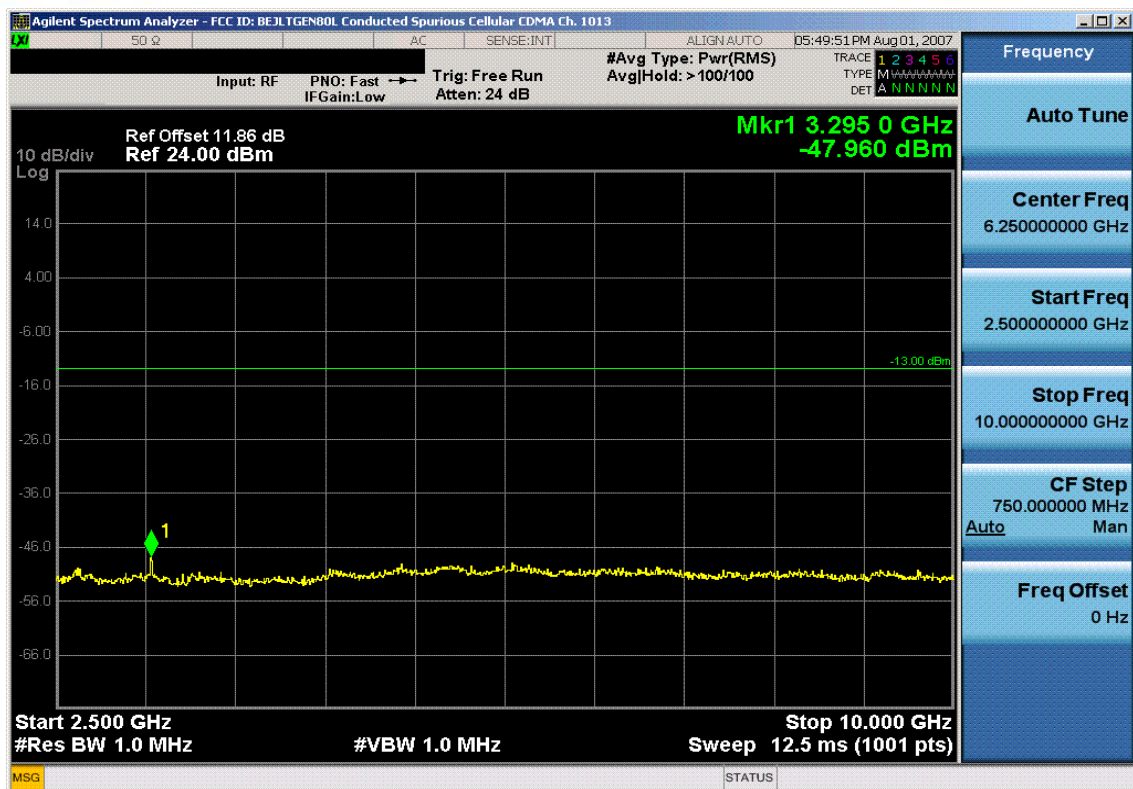
Plot 7-17. Conducted Spurious Plot (Cellular CDMA Mode – Ch. 1013)
