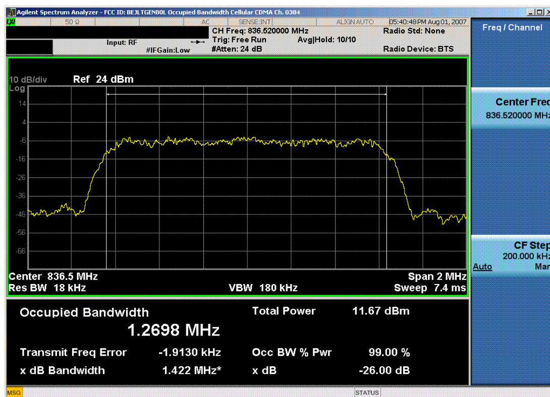
Plot 7-22. Occupied Bandwidth Plot (Cellular CDMA Mode – Ch. 384)
