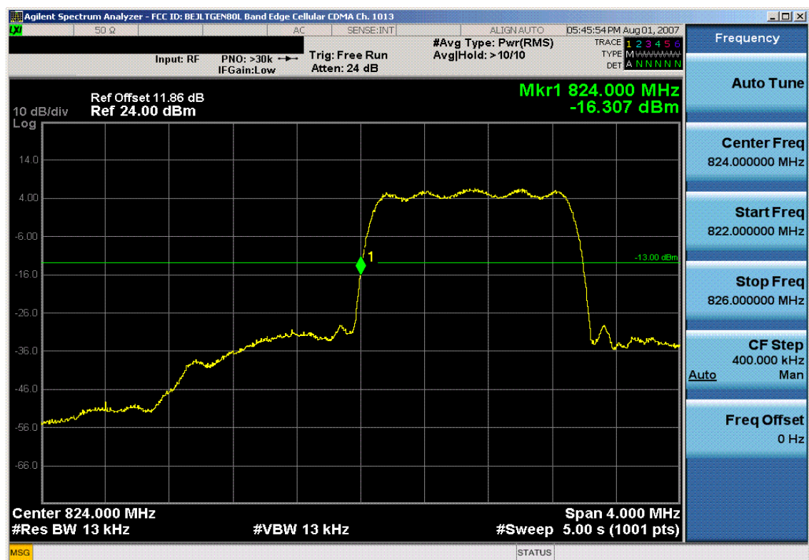
Plot 7-18. Band Edge Plot (Cellular CDMA Mode – Ch. 1013)
