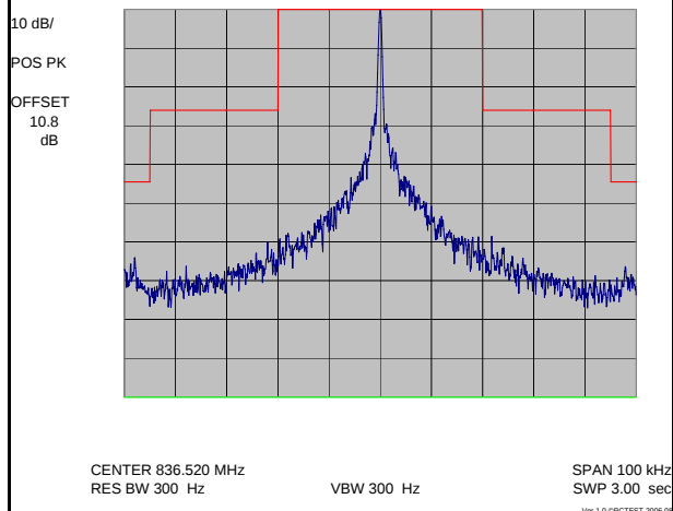
Plot 7-10. Unmodulated Signal
