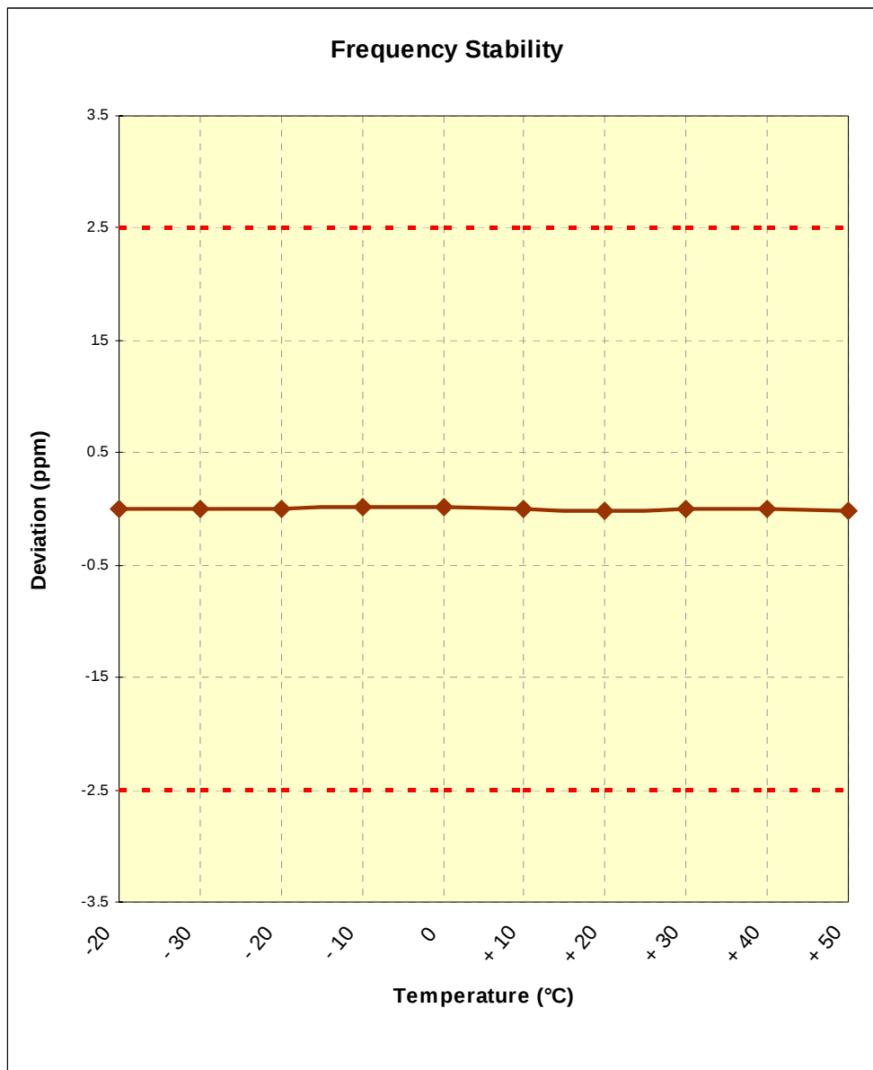
Figure 6-2. Frequency Stability Graph (AMPS Mode – Ch.384)
