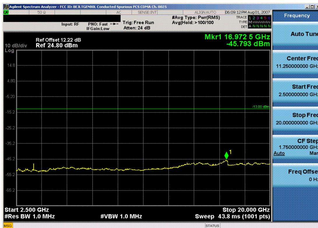
Plot 7-28. Conducted Spurious Plot (PCS CDMA Mode – Ch. 25)
