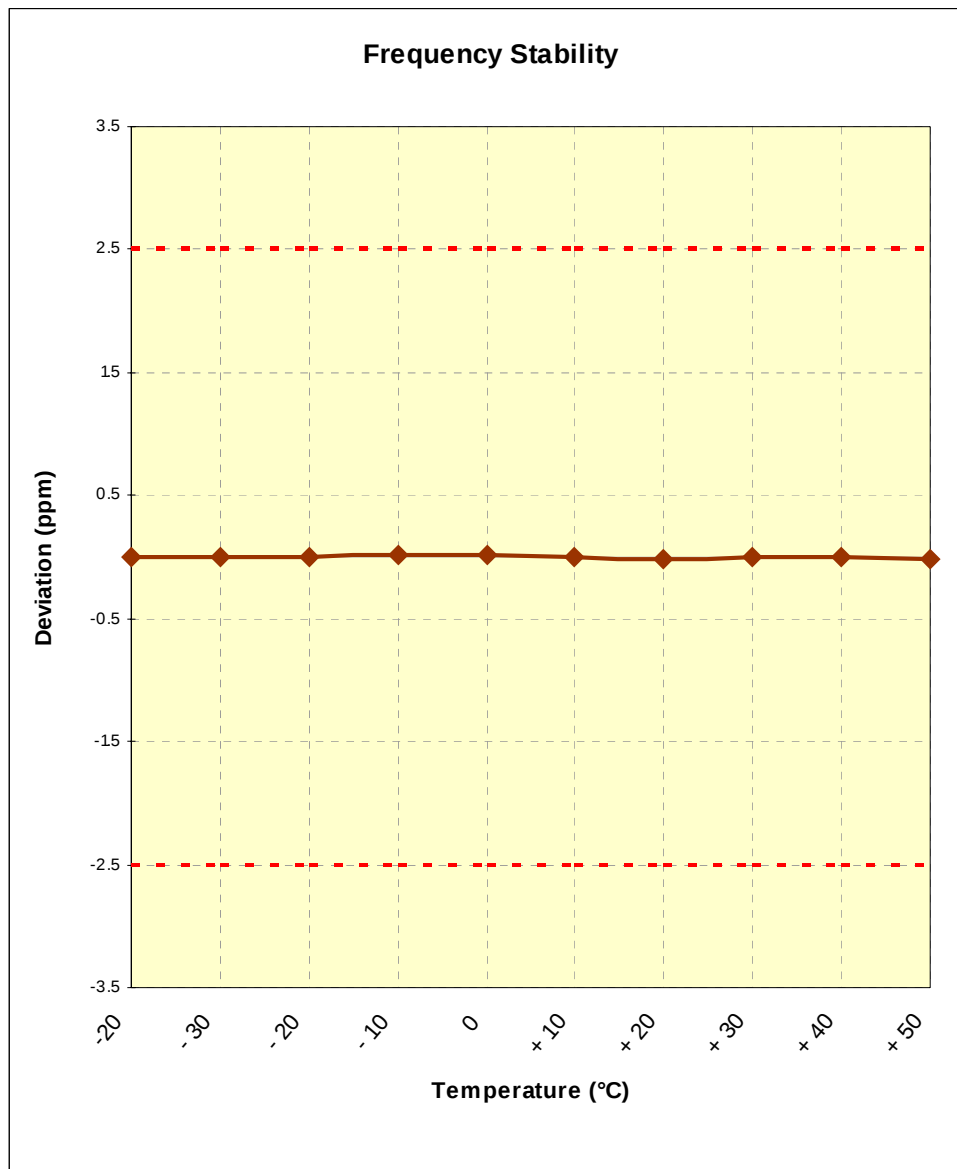
Figure 6-3. Frequency Stability Graph (Cellular CDMA Mode – Ch. 384)
