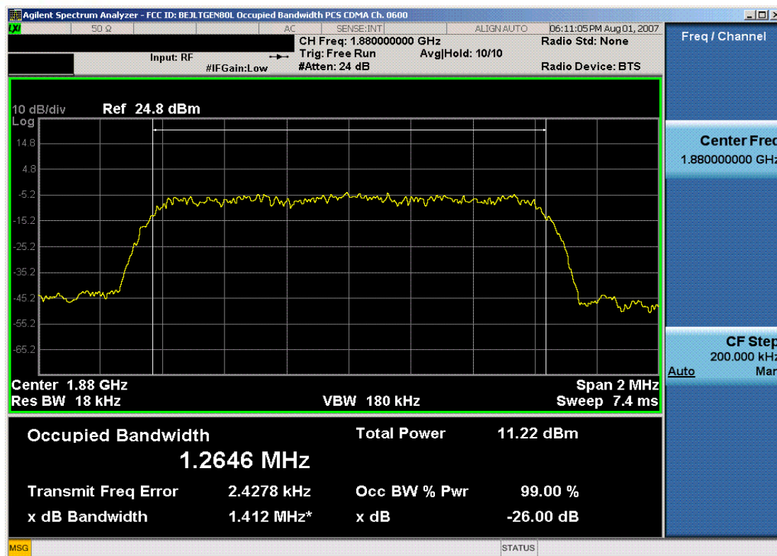
Plot 7-33. Occupied Bandwidth Plot (PCS CDMA Mode – Ch. 600)
