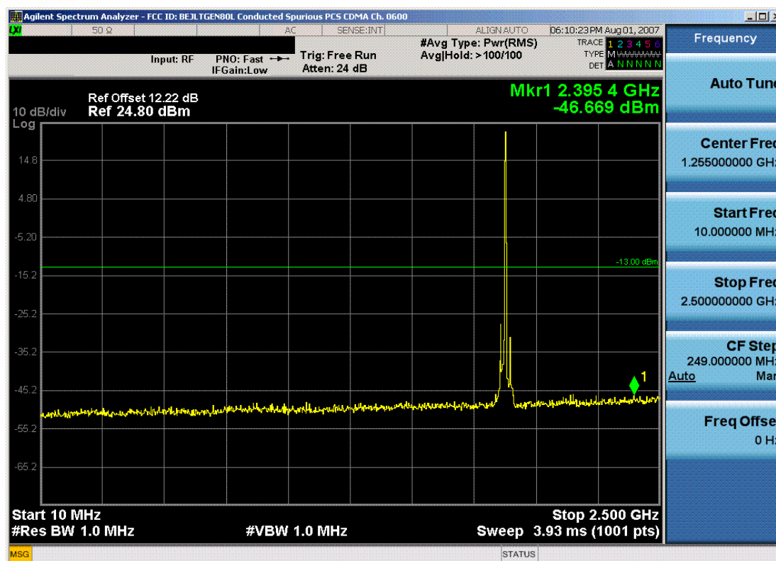
Plot 7-31. Conducted Spurious Plot (PCS CDMA Mode – Ch. 600)
