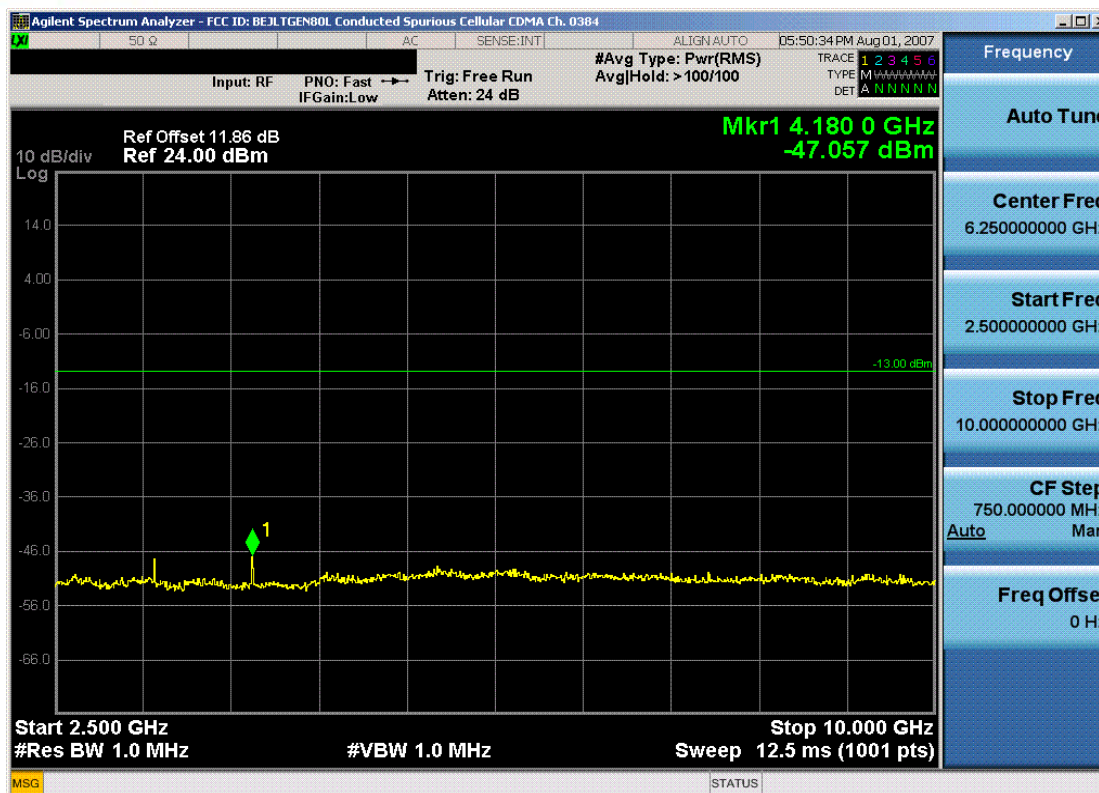
Plot 7-21. Conducted Spurious Plot (Cellular CDMA Mode – Ch. 384)
