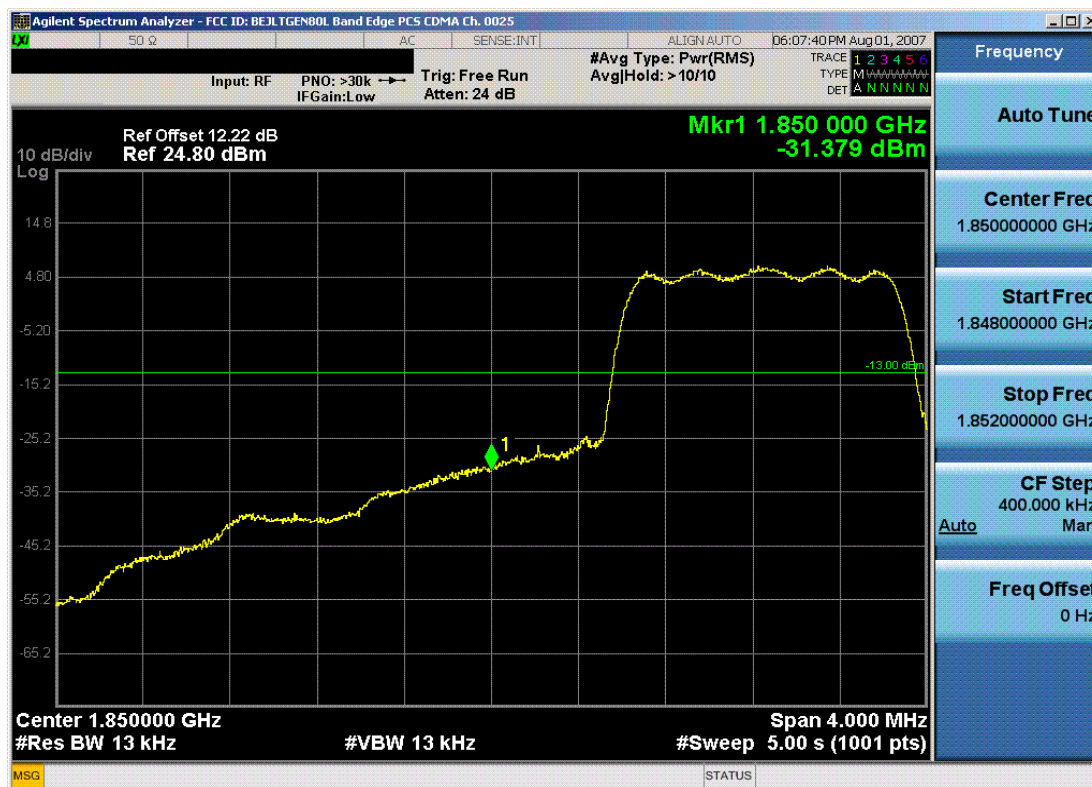
Plot 7-29. Band Edge Plot (PCS CDMA Mode – Ch. 25)
