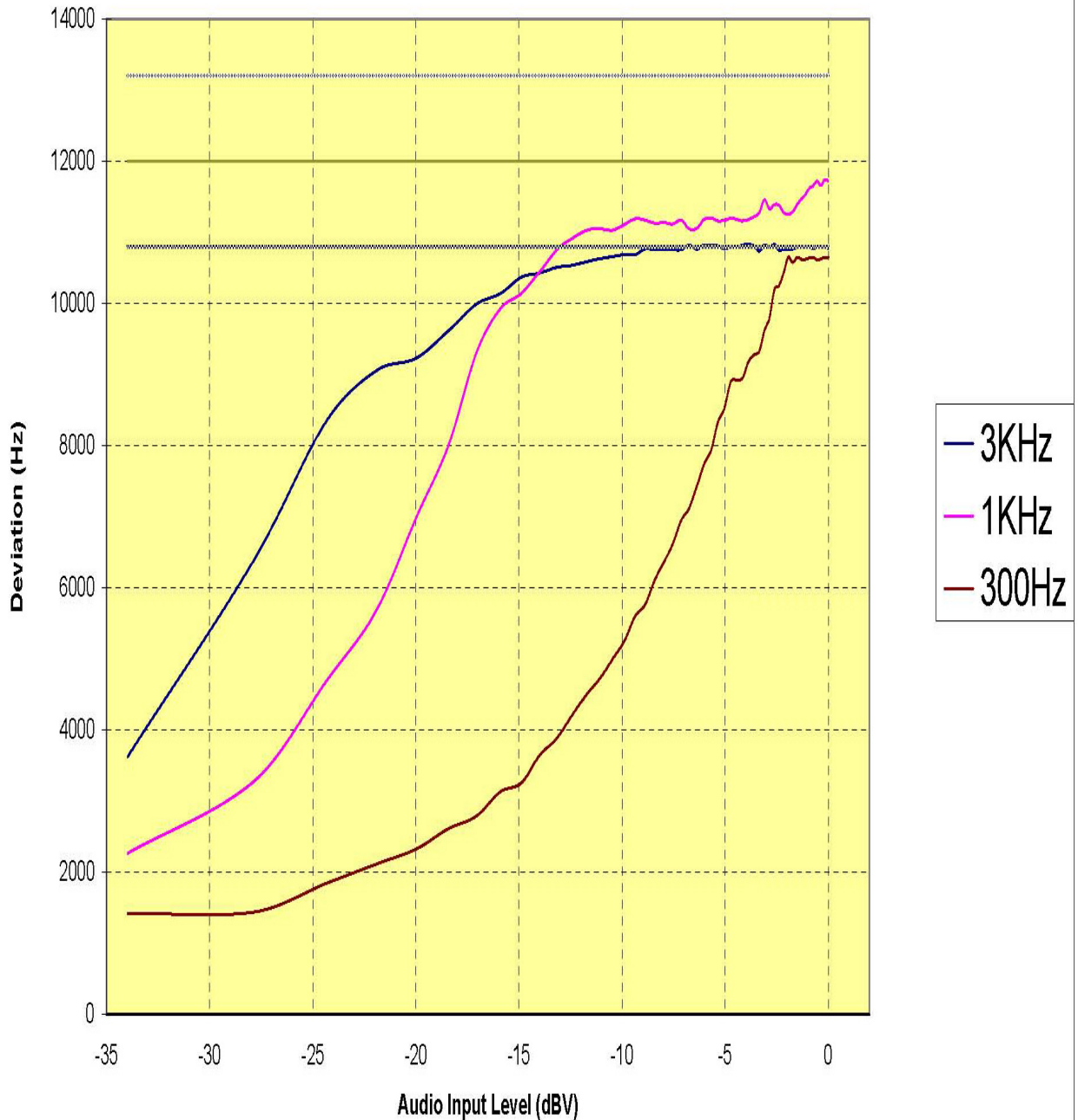
Plot 7-7. Modulation Limiting Plot (AMPS Mode – Ch. 384)
