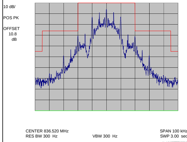
Plot 7-13. Wide Band Data Signal (WBD)
