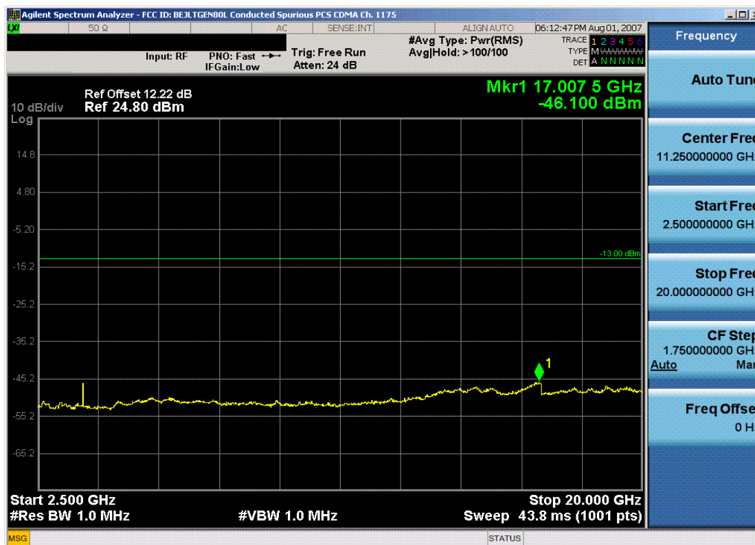
Plot 7-35. Conducted Spurious Plot (PCS CDMA Mode – Ch. 1175)
