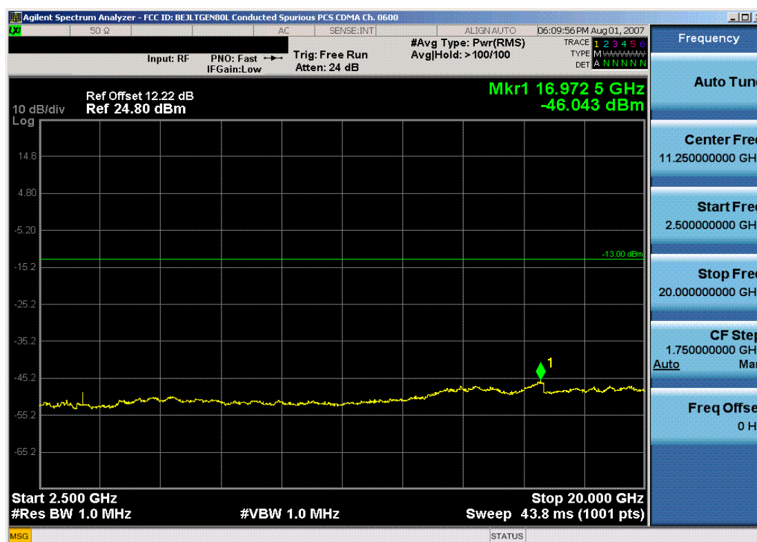
Plot 7-32. Conducted Spurious Plot (PCS CDMA Mode – Ch. 600)
