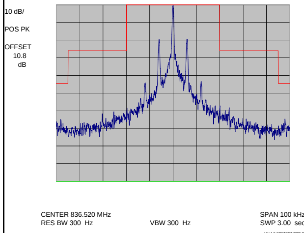
Plot 7-12. Supervisory Audio Tone (SAT)
