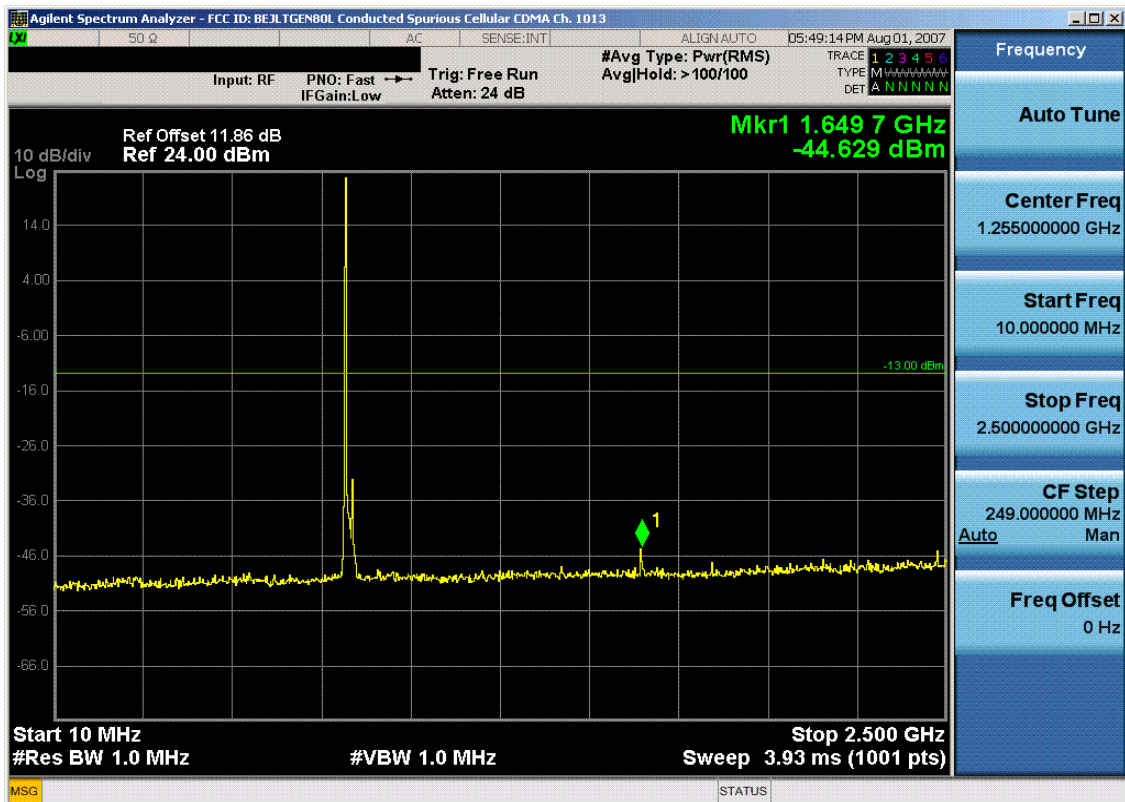
Plot 7-16. Conducted Spurious Plot (Cellular CDMA Mode – Ch. 1013)
