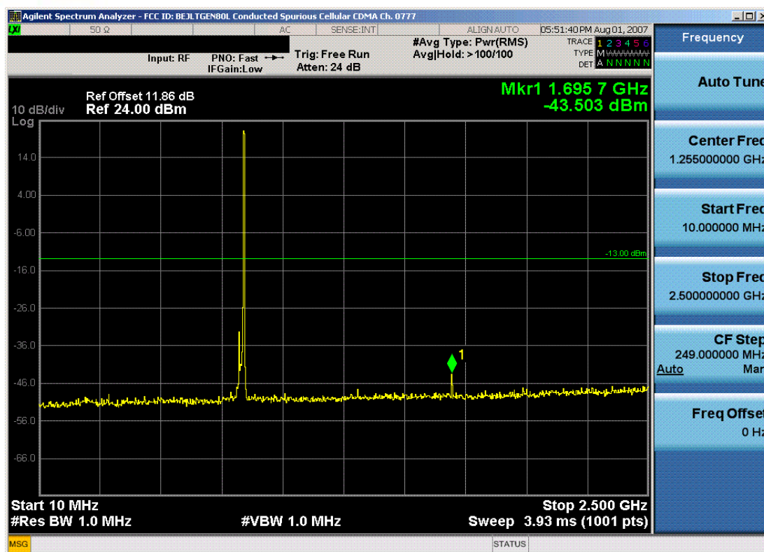
Plot 7-23. Conducted Spurious Plot (Cellular CDMA Mode – Ch. 777)
