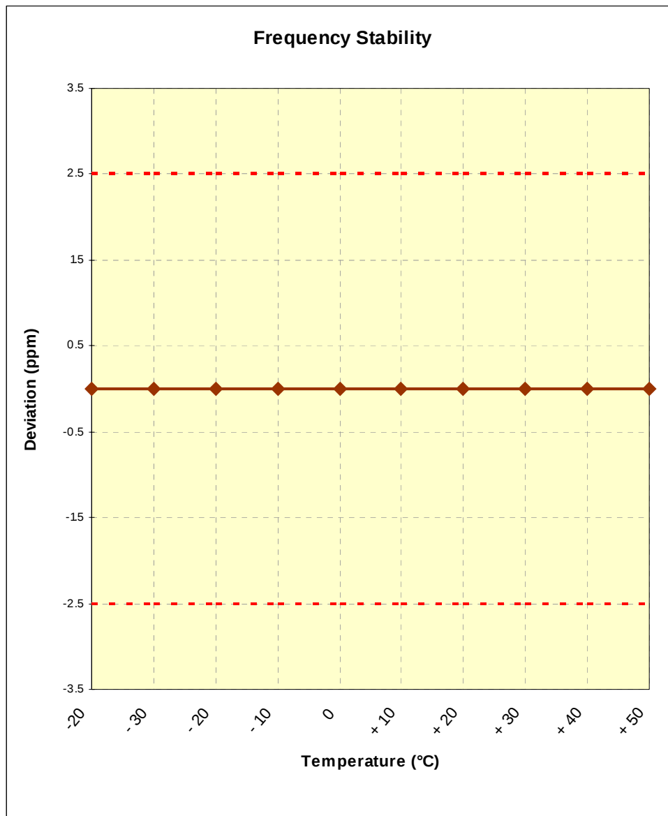
Figure 6-4. Frequency Stability Graph (PCS CDMA Mode – Ch. 600)
