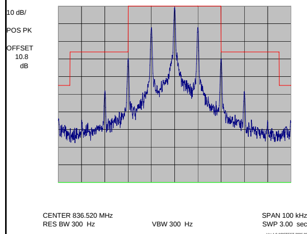
Plot 7-11. Signaling Tone (ST)
