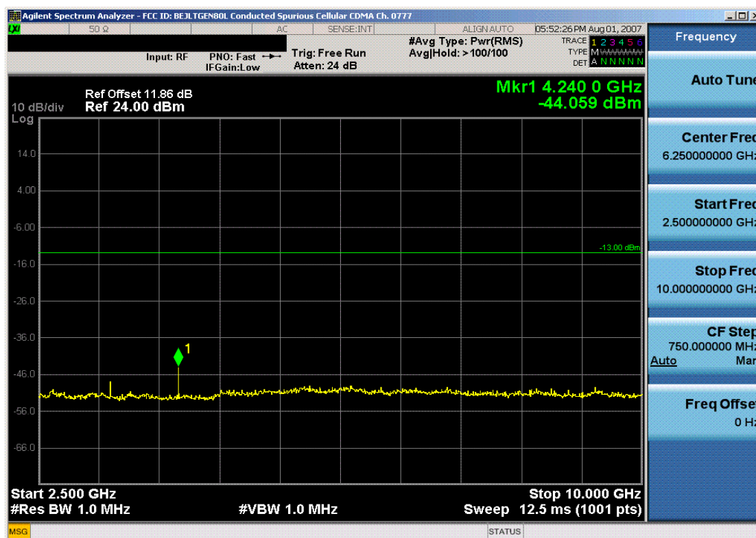
Plot 7-24. Conducted Spurious Plot (Cellular CDMA Mode – Ch. 777)
