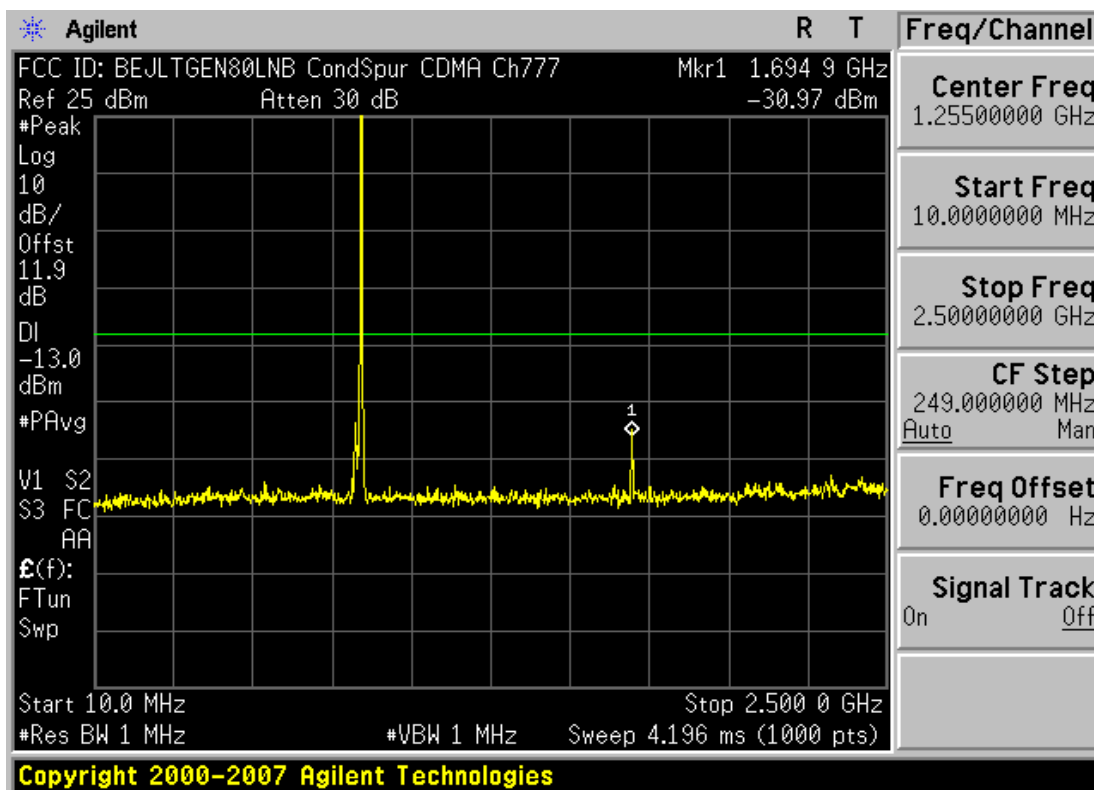
Plot 7-16. Conducted Spurious Plot (Cellular CDMA Mode – Ch. 777)
