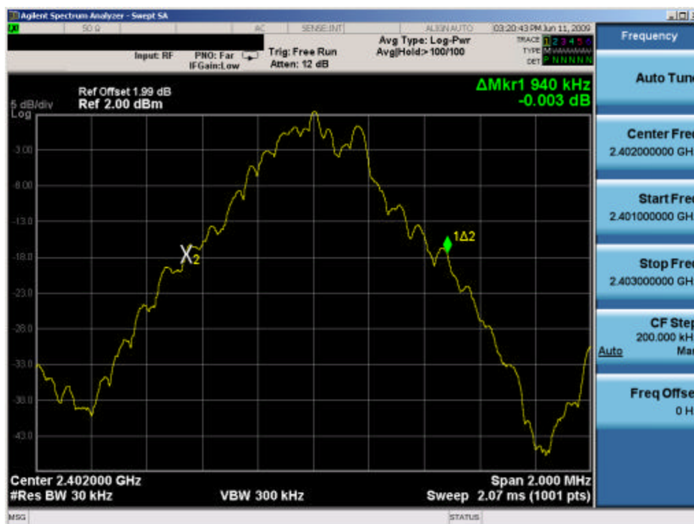
Plot 6-1. 20dB Bandwidth Plot (Bluetooth 1.0 – Ch. 0)
