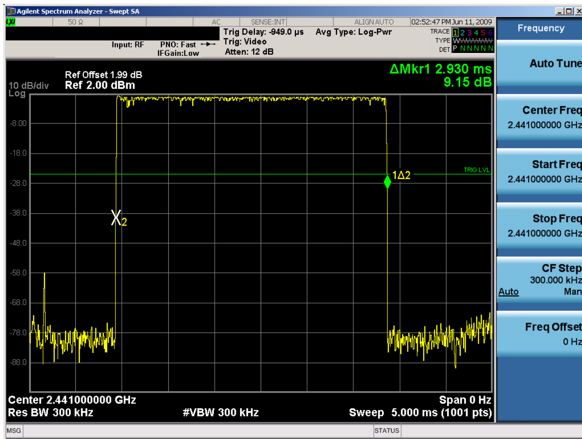
Plot 6-1. Time of Occupancy Plot (Bluetooth)
