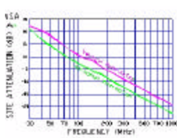
Figure 3-4. Normalized Site Attenuation Curves (H&V)
