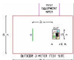
Figure 3-2. Dimensions of Outdoor Test Site
