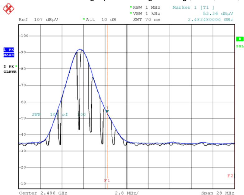
Radiated Restricted Band Edges plot – Average Reading (8DPSK, Ch.78, X-H)
