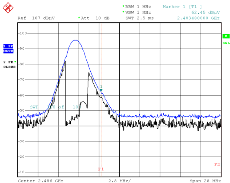
Radiated Restricted Band Edges plot – Peak Reading (8DPSK, Ch.78, X-H)
