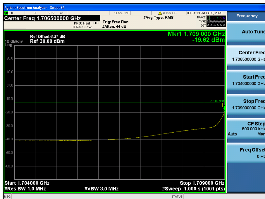
LTE Band 4 / 1.4MHz / QPSK - RB Size/Offset (1/2)
