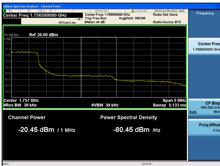
LTE Band 4 / 5MHz / QPSK - RB Size/Offset (25/25)
