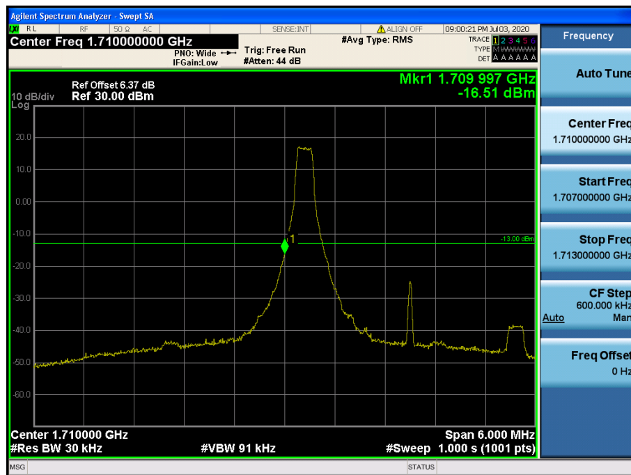
LTE Band 4 / 3MHz / 16QAM - RB Size/Offset (1/0)
