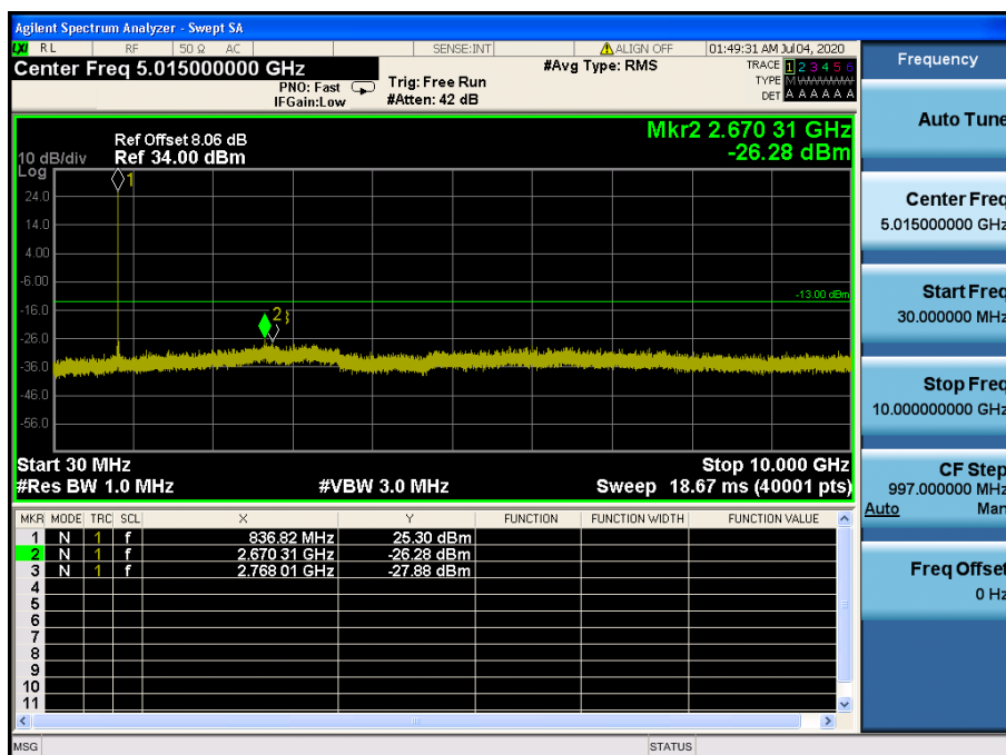
LTE Band 5 / 3MHz / QPSK - RB Size/Offset (8/7) – Mid Channel
