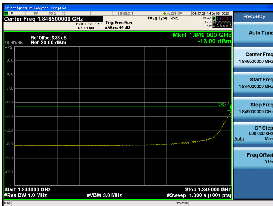
LTE Band 2 / 1.4MHz / 16QAM - RB Size/Offset (3/2)
