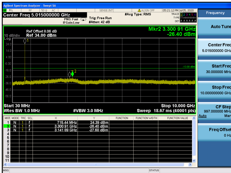
LTE Band 17 / 5MHz / 16QAM - RB Size/Offset (12/13) – High Channel
