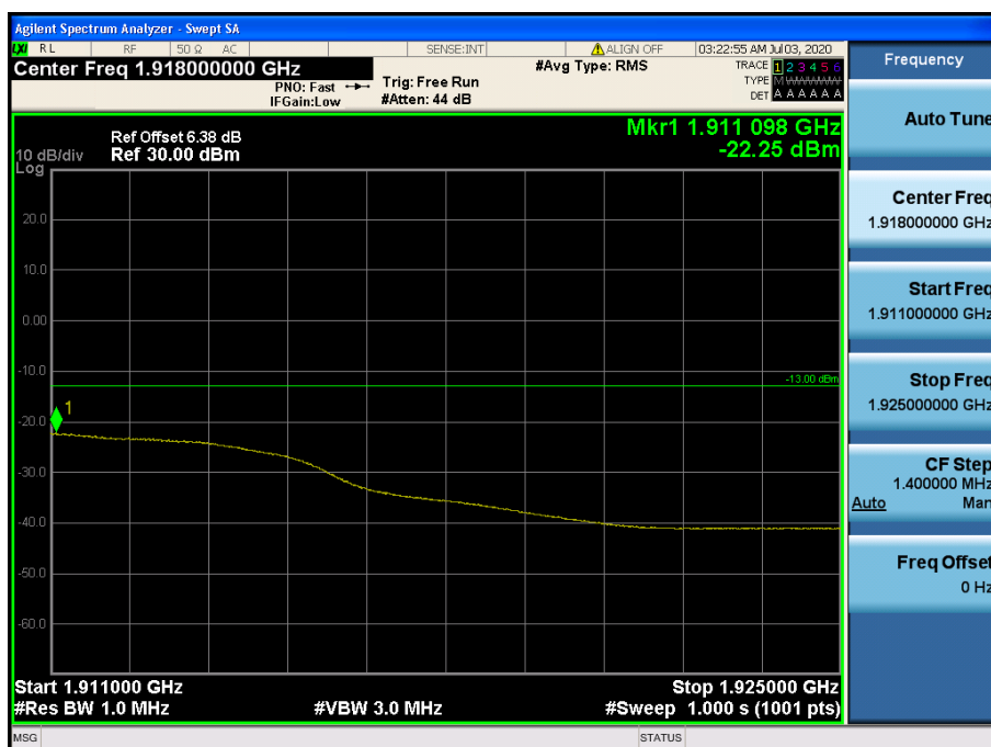
LTE Band 2 / 15MHz / QPSK - RB Size/Offset (36/39)
