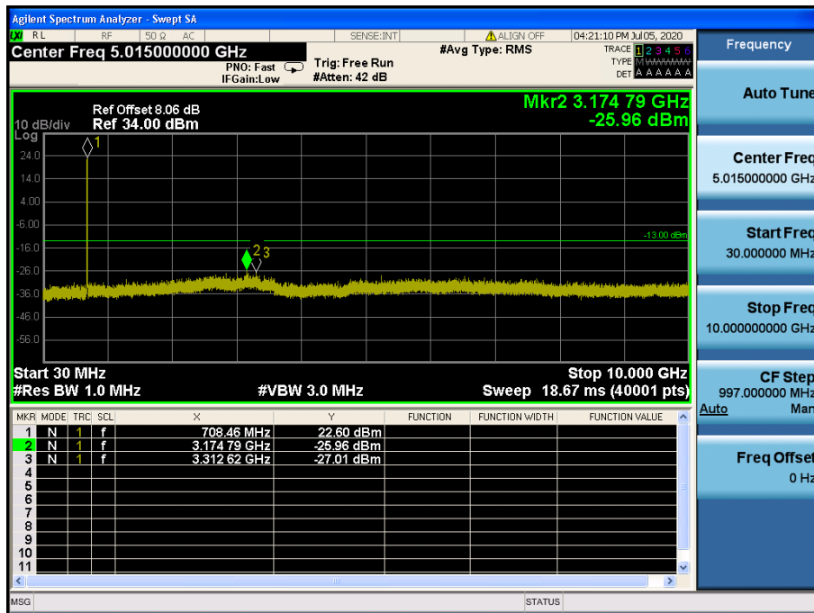
LTE Band 17 / 10MHz / QPSK - RB Size/Offset (25/0) – Low Channel
