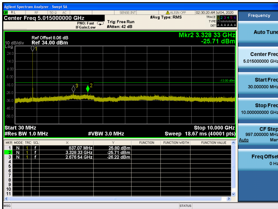
LTE Band 5 / 5MHz / QPSK - RB Size/Offset (1/12) – Mid Channel
