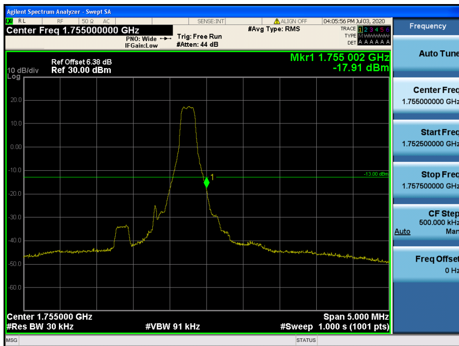
LTE Band 4 / 1.4MHz / QPSK - RB Size/Offset (1/5)
