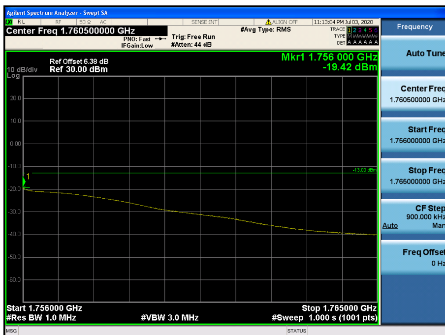
LTE Band 4 / 10MHz / 16QAM - RB Size/Offset (25/25)
