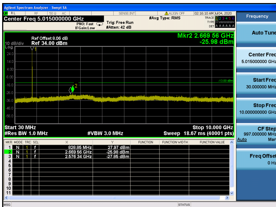
LTE Band 5 / 5MHz / QPSK - RB Size/Offset (1/24) – Low Channel
