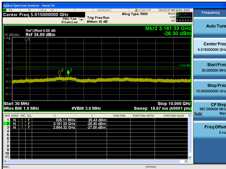
LTE Band 5 / 3MHz / 16QAM - RB Size/Offset (8/0) – Low Channel
