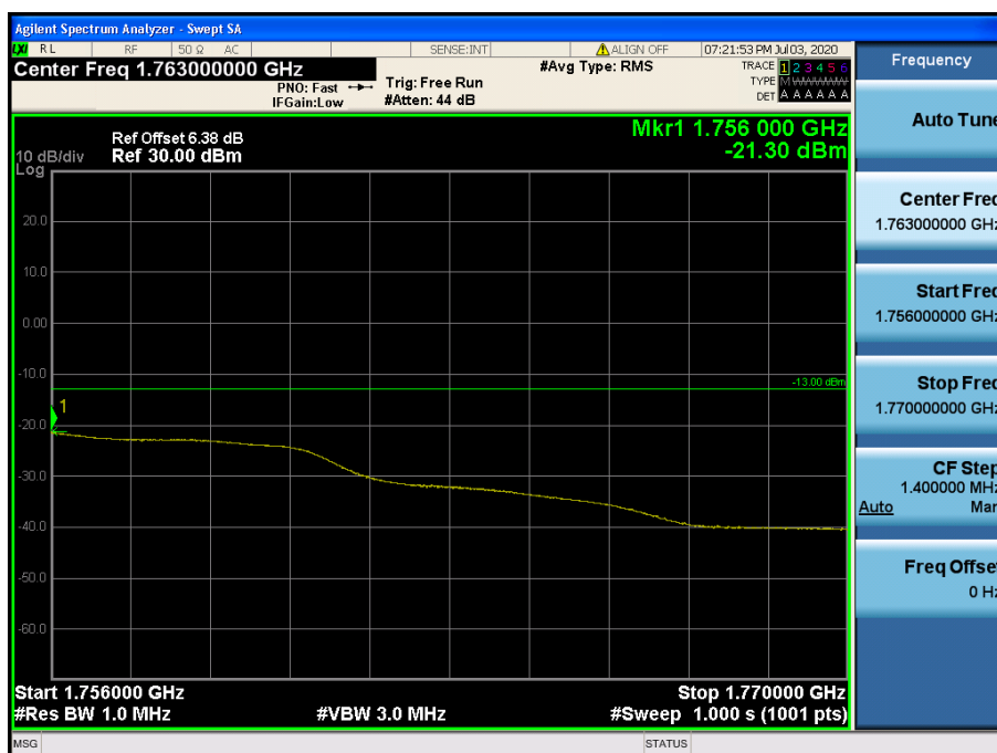
LTE Band 4 / 15MHz / 16QAM - RB Size/Offset (36/39)
