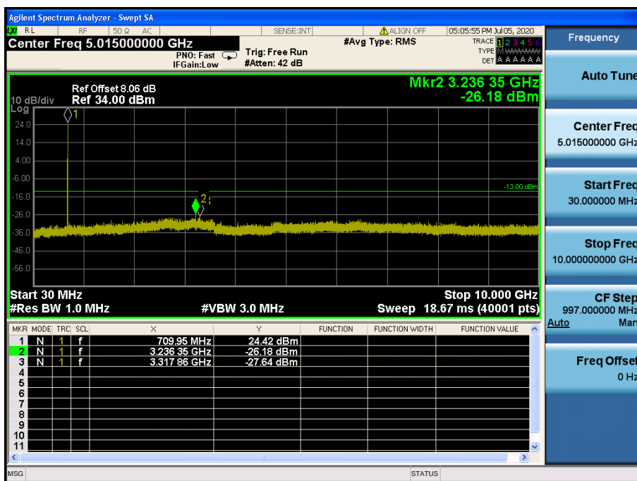
LTE Band 17 / 5MHz / 16QAM - RB Size/Offset (12/6) – Mid Channel
