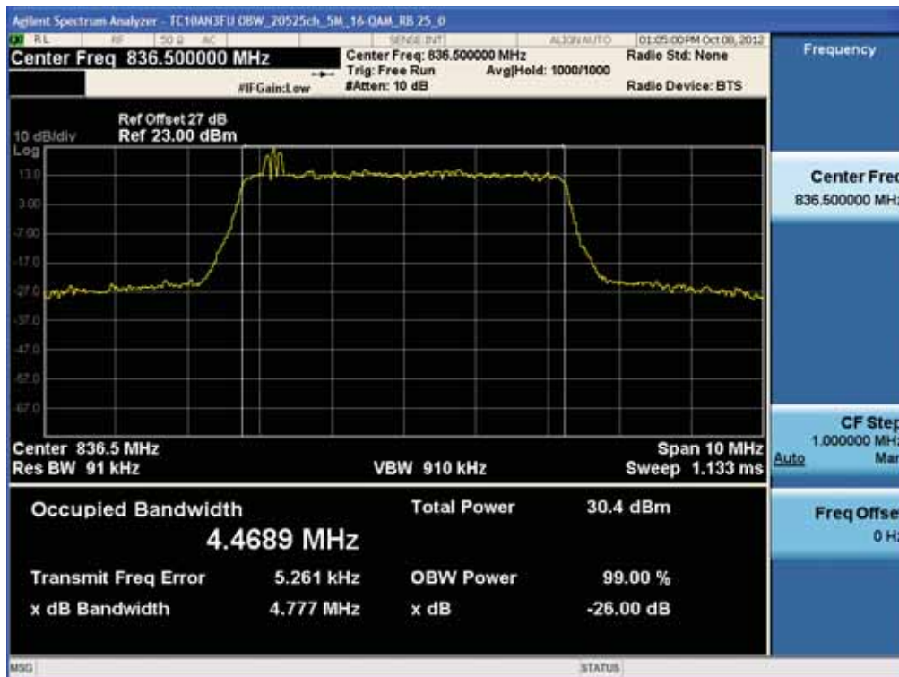
BAND 5. Occupied Bandwidth Plot (20525ch_5MHz_16-QAM_RB 25_0)
