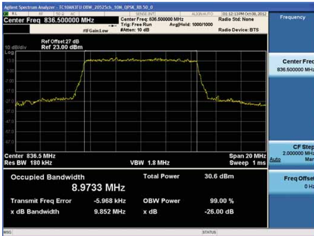
BAND 5. Occupied Bandwidth Plot (20525ch_10MHz_QPSK_RB 50_0)
