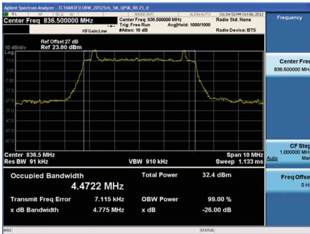
BAND 5. Occupied Bandwidth Plot (20525ch_5MHz_QPSK_RB 25_0)
