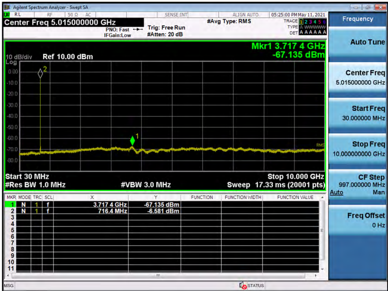
BAND 17. Conducted Spurious Plot _ (23825ch_5MHz_QPSK_RB 1_0)
