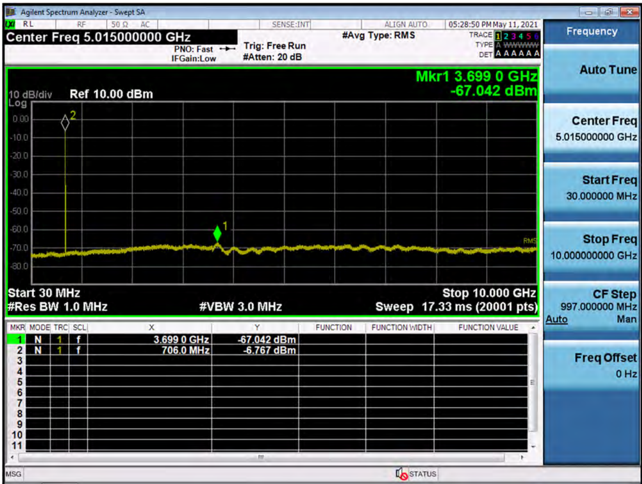
BAND 17. Conducted Spurious Plot _ (23790ch_10MHz_QPSK_RB 1_0)
