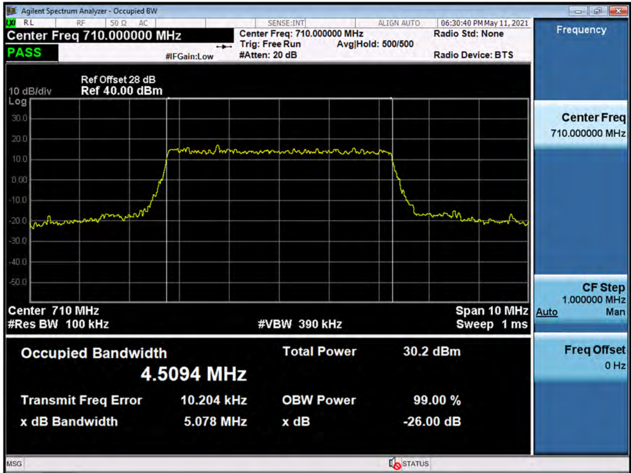
BAND 17. Occupied Bandwidth Plot (5M BW Ch.23790 QPSK_RB25_0)
