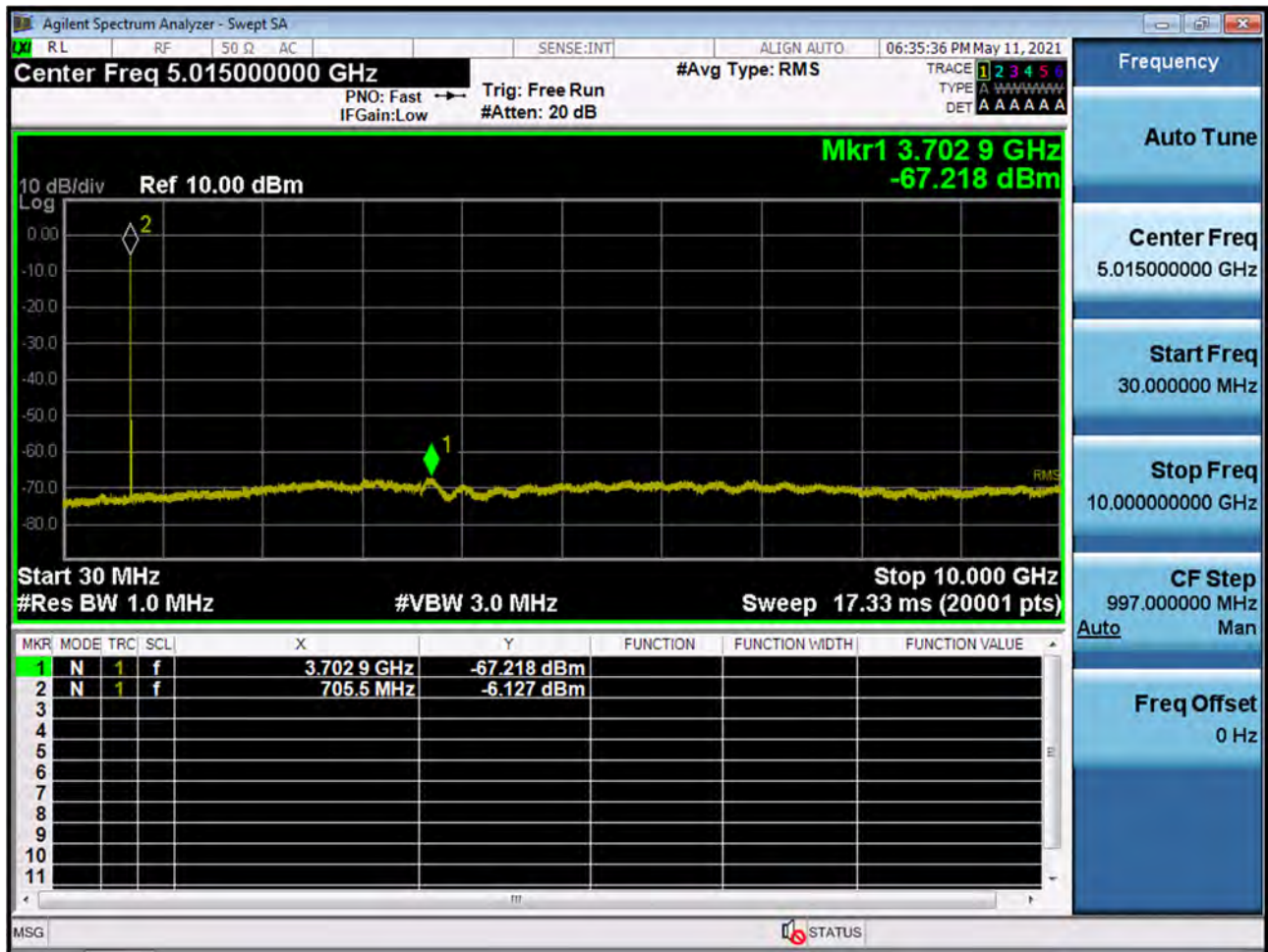
BAND 17. Conducted Spurious Plot _ (23780ch_10MHz_QPSK_RB 1_0)
