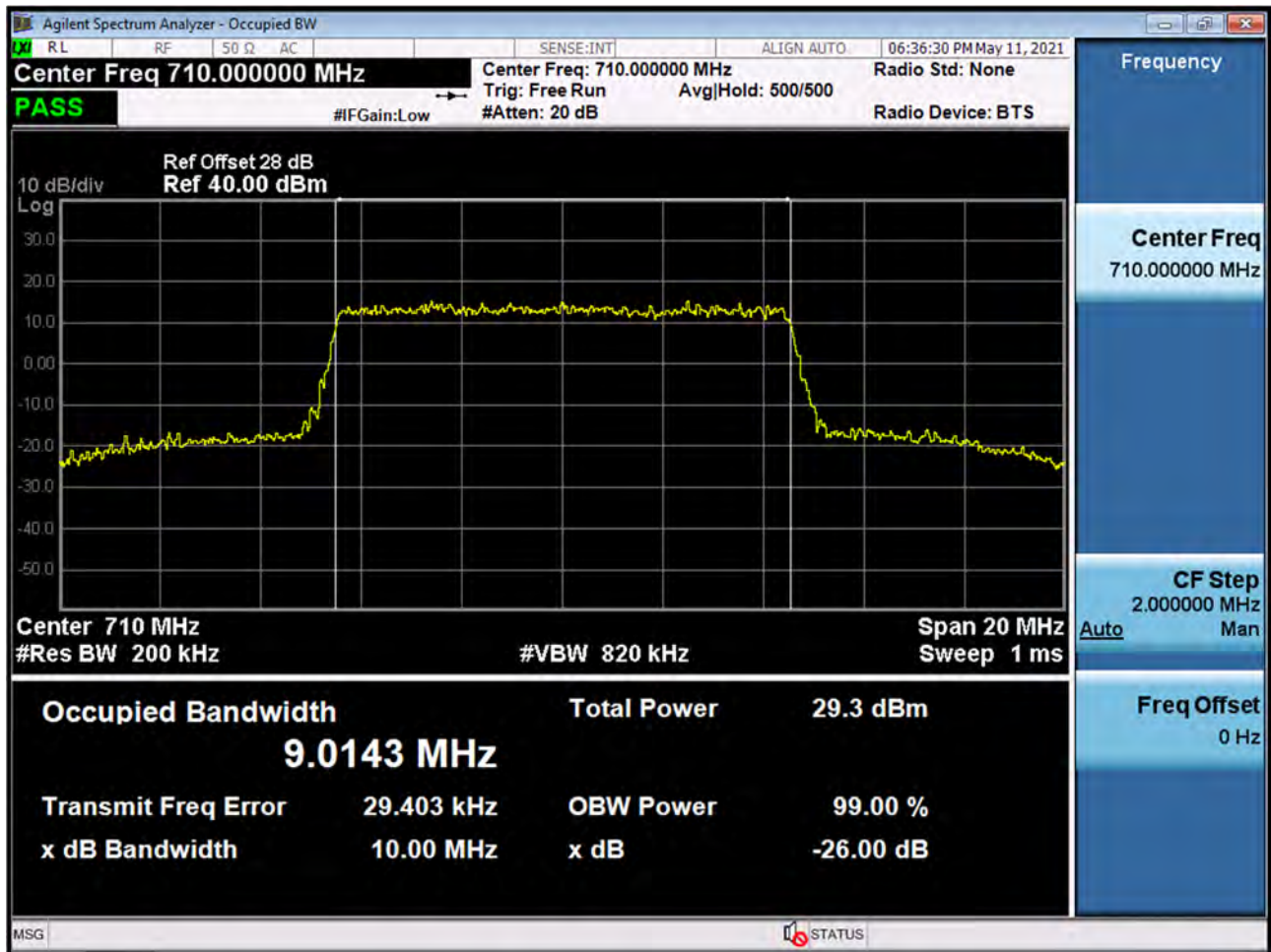
BAND 17. Occupied Bandwidth Plot (10M BW Ch.23790 16QAM_RB50_0)
