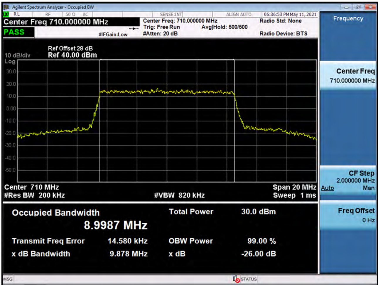
BAND 17. Occupied Bandwidth Plot (10M BW Ch.23790 QPSK_RB50_0)
