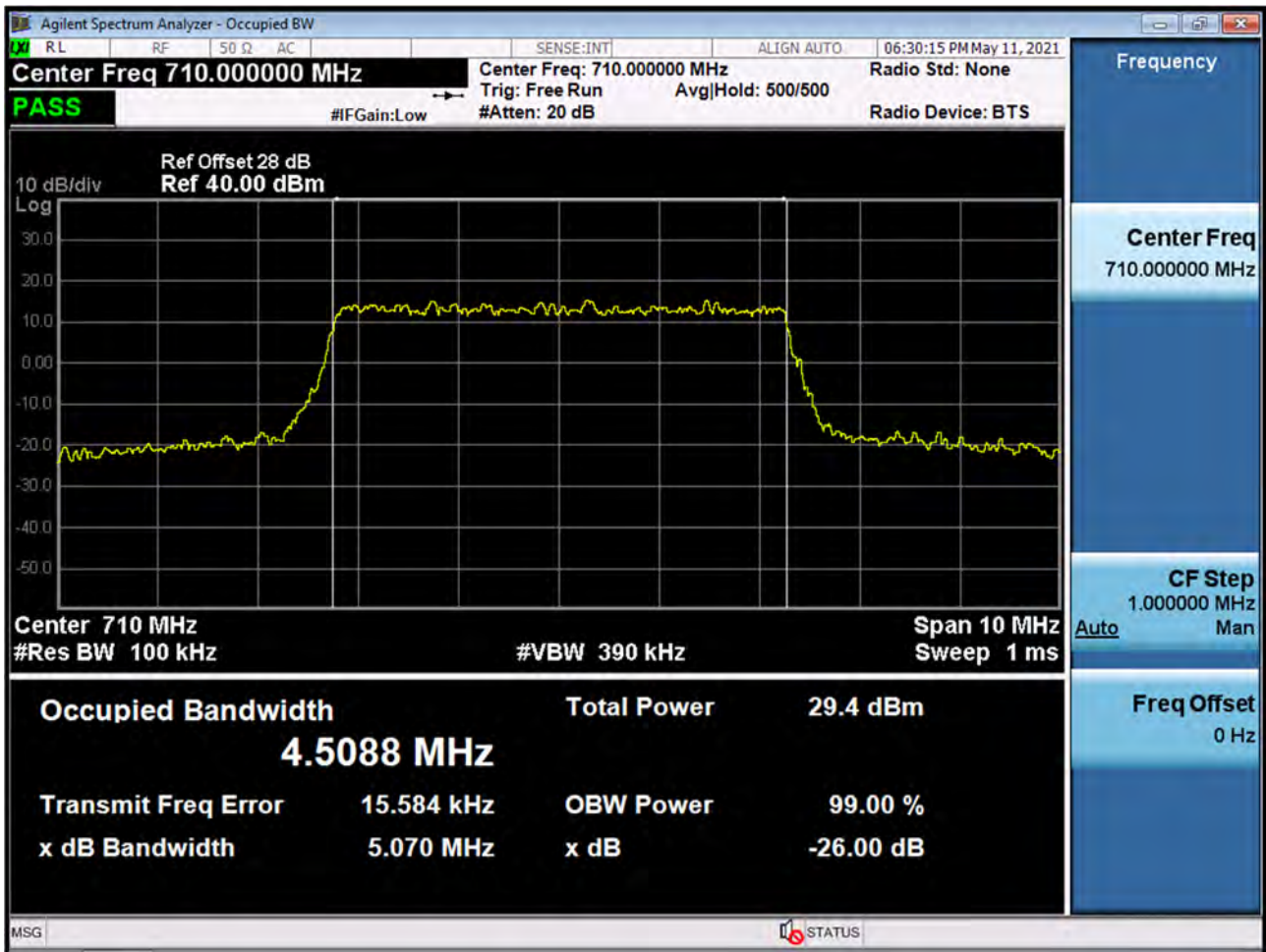
BAND 17. Occupied Bandwidth Plot (5M BW Ch.23790 16QAM_RB25_0)
