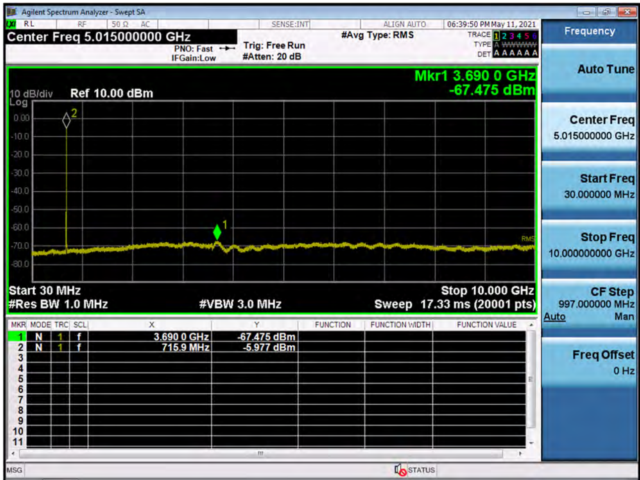
BAND 17. Conducted Spurious Plot _ (23800ch_10MHz_QPSK_RB 1_0)
