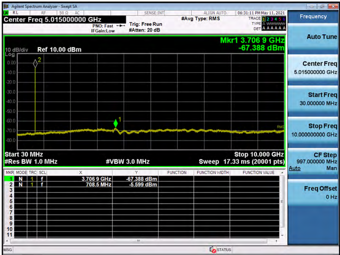
BAND 17. Conducted Spurious Plot _ (23790ch_5MHz_QPSK_RB 1_0)
