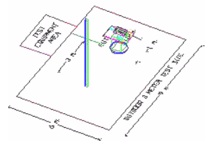
Figure 3-3. Turntable and System Setup
