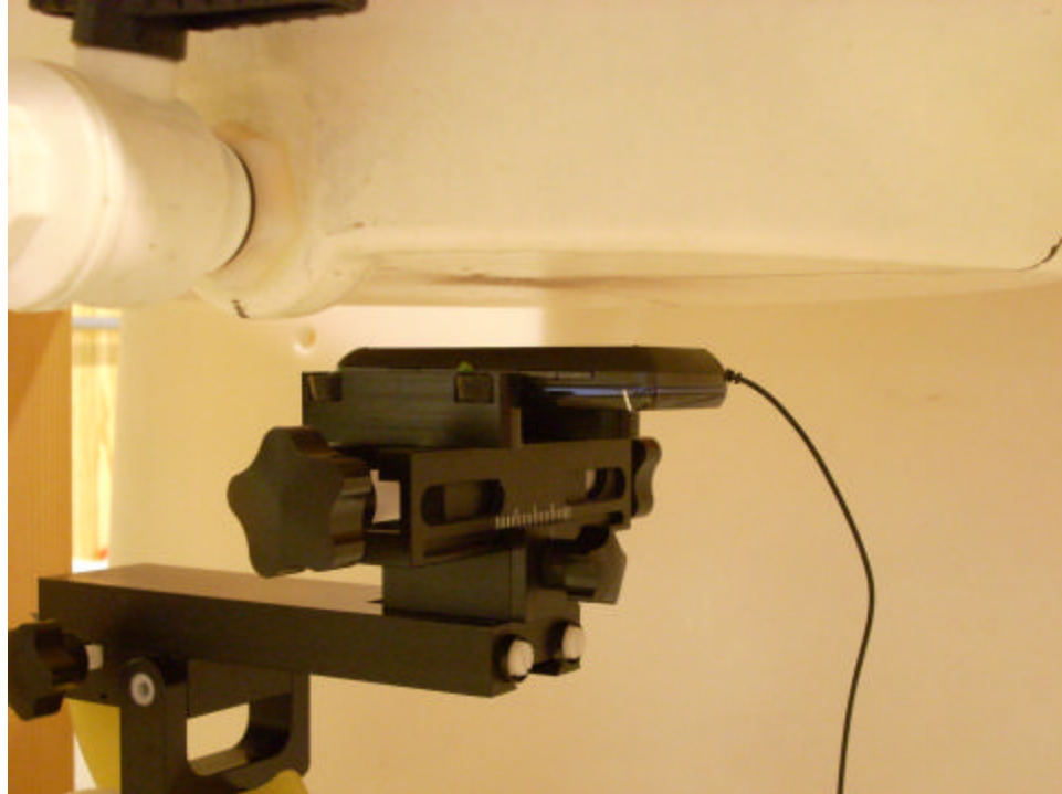
Figure 1-5 SAR Test Setup Photo 5
