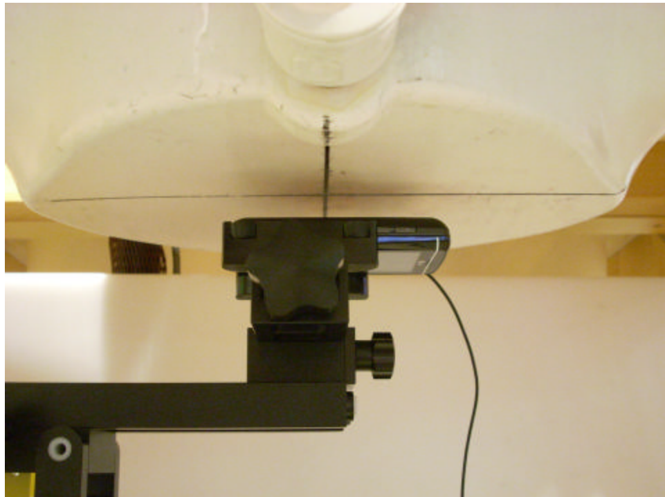
Figure 1-6 SAR Test Setup Photo 6
