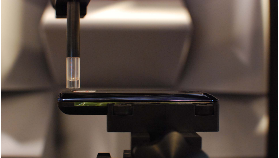
Figure 13-1 Test Setup for Wireless Device
