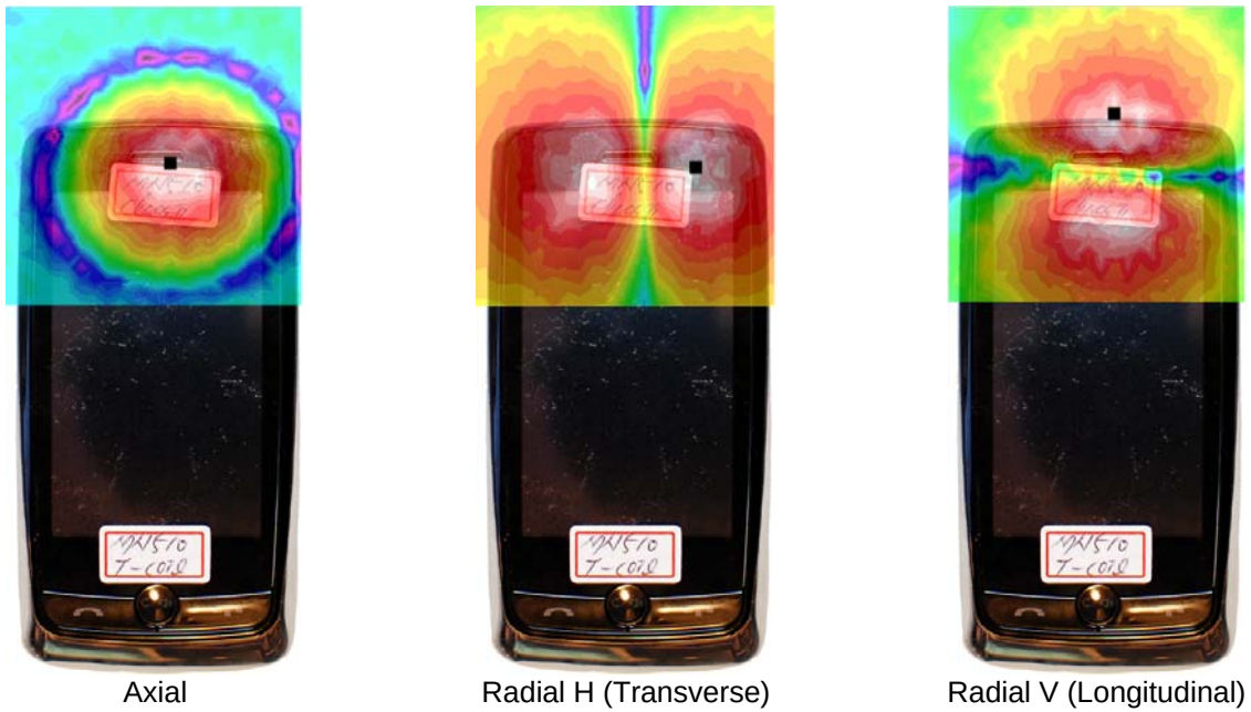
Figure 13-3 T-Coil Scan Overlay Magnetic Field Distributions
