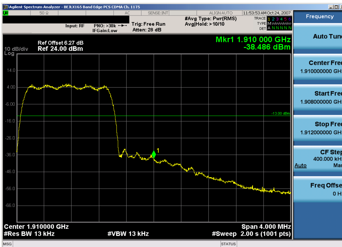
Plot 7-10. Band Edge Plot (PCS CDMA Mode – Ch. 1175)
