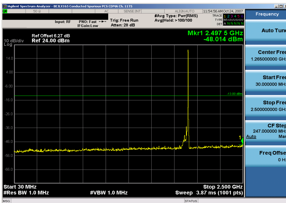
Plot 7-8. Conducted Spurious Plot (PCS CDMA Mode – Ch. 1175)
