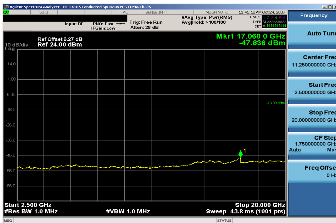
Plot 7-2. Conducted Spurious Plot (PCS CDMA Mode – Ch. 25)
