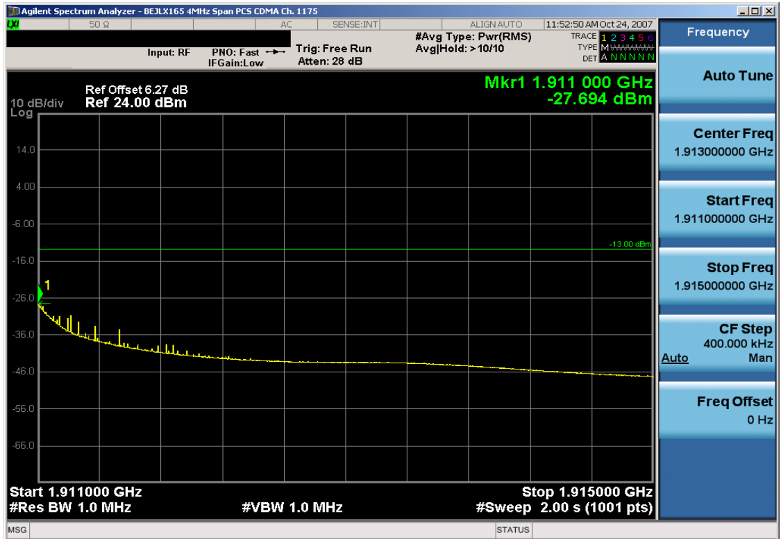
Plot 7-11. 4MHz Span Plot (PCS CDMA Mode – Ch. 1175)
