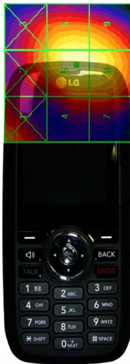
Figure 17-4 E-Field WD Scan overlay
