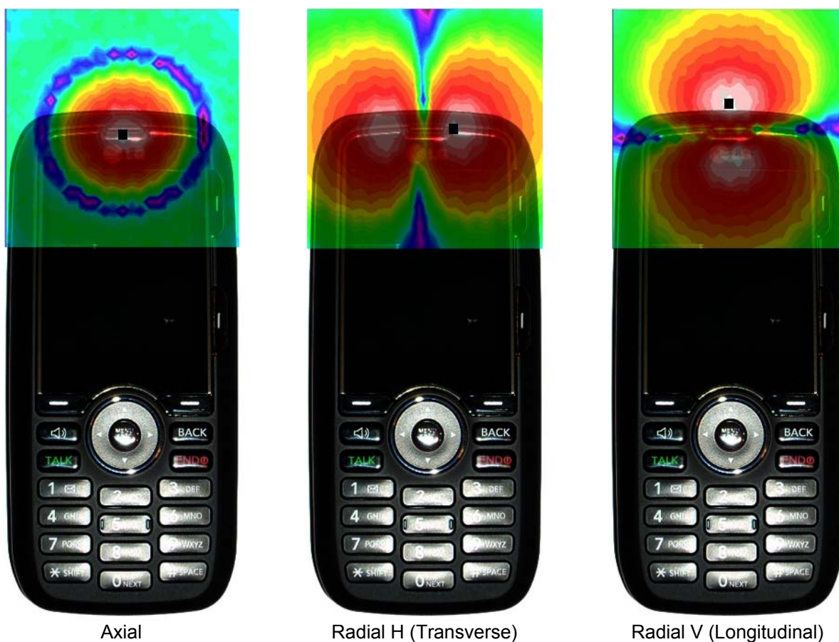
Figure 13-3 T-Coil Scan Overlay Magnetic Field Distributions
