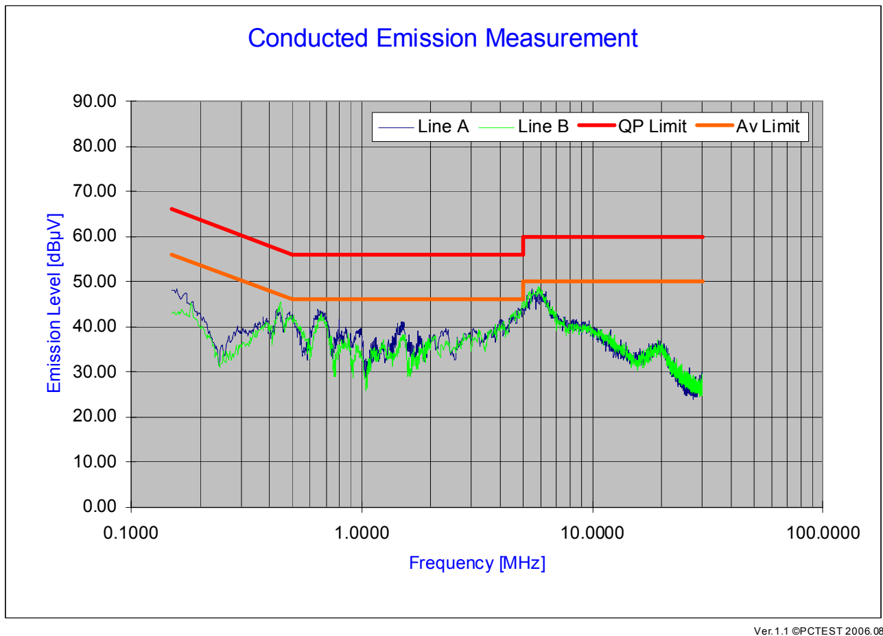
Plot 6-1. Line Conducted Plot with Bluetooth
