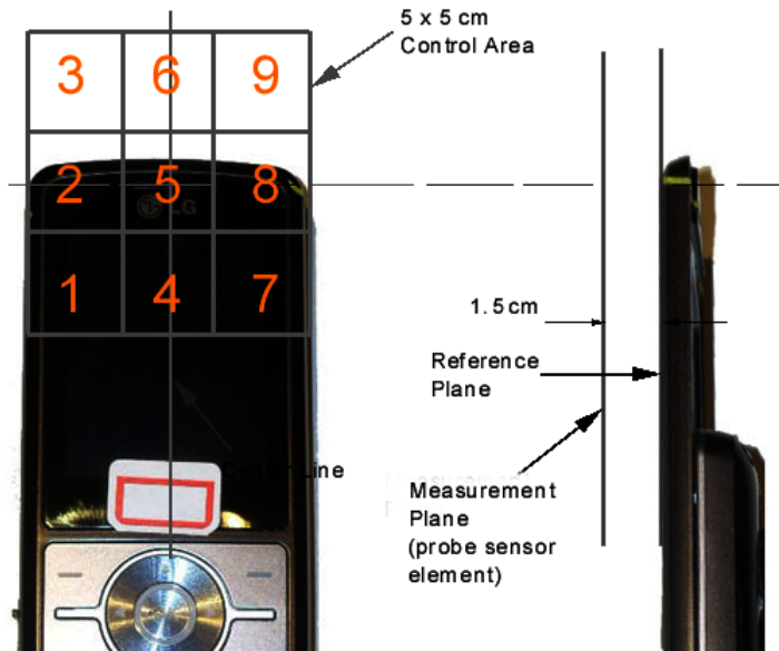
Figure 17-3 5x5 Scan grid above WD
