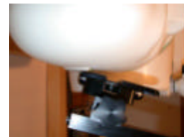
Figure 14.14 Right Head SAR Test Setup -- Ear / Tilt Position --
