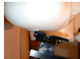
Figure 14.22 Right Head SAR Test Setup -- Ear / Tilt Position --
