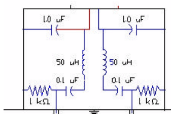
Figure 5. LISN Schematic Diagram
