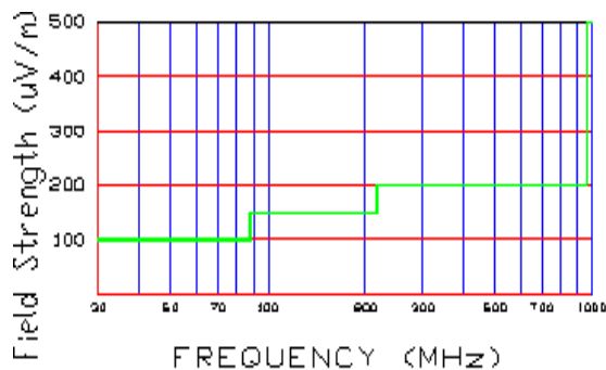
Figure 11. Spurious Radiated Limits at 3 meters
