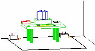
Figure 3. Line Conducted Emission Test Set-Up
