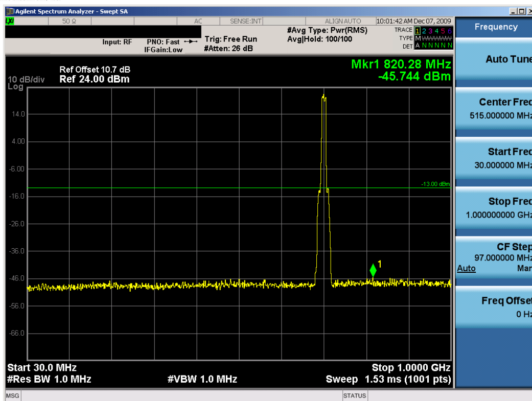
Plot 7-11. Conducted Spurious Plot (16-QAM Modulation – 709MHz)
