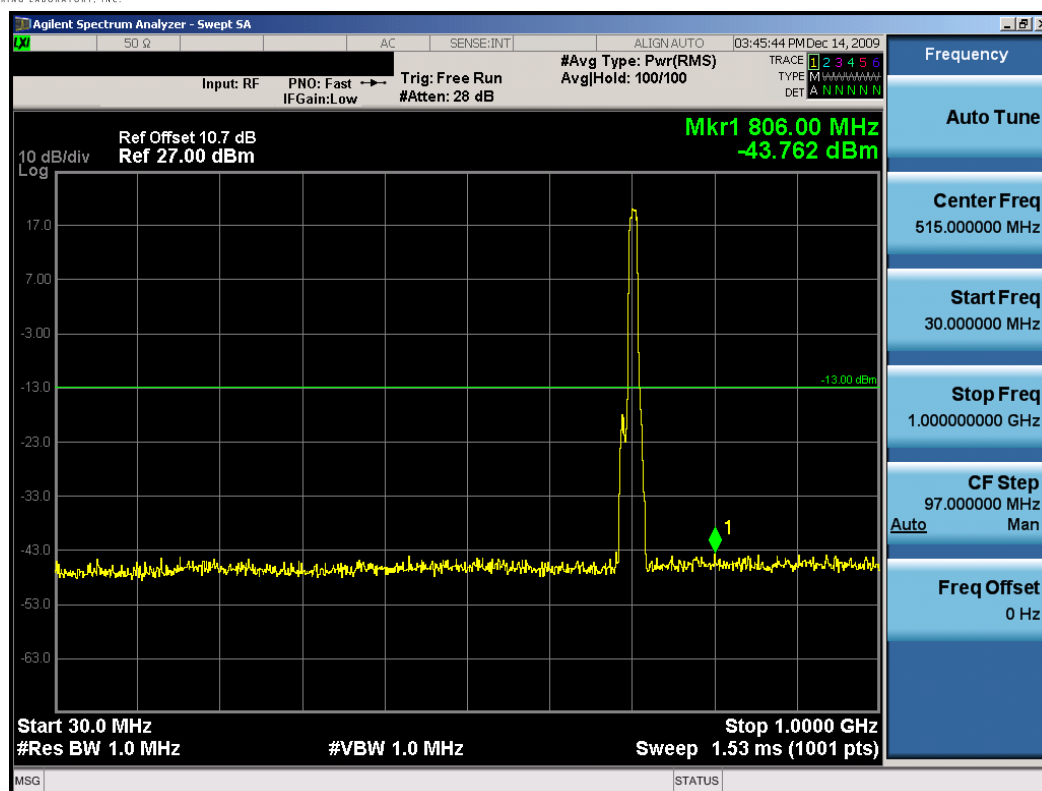
Plot 7-21. Conducted Spurious Plot (QPSK Modulation – 711MHz)
