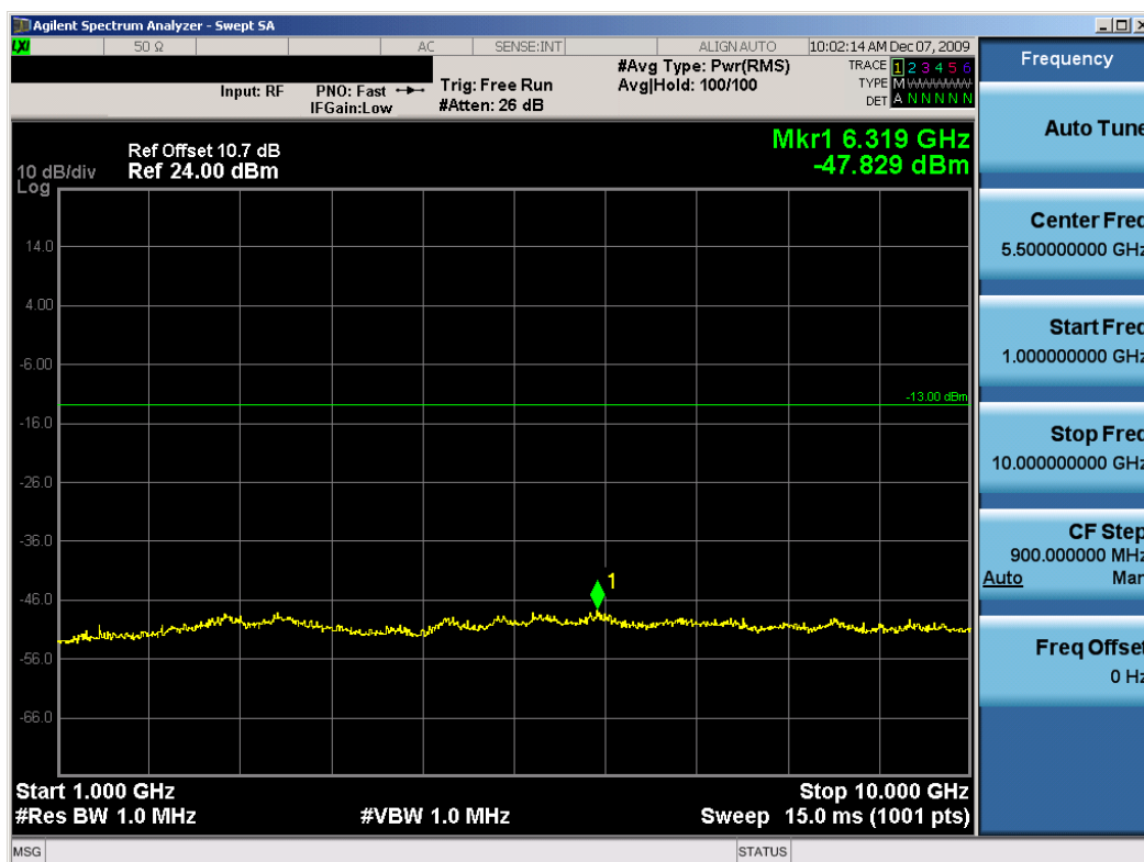
Plot 7-12. Conducted Spurious Plot (16-QAM Modulation – 709MHz)
