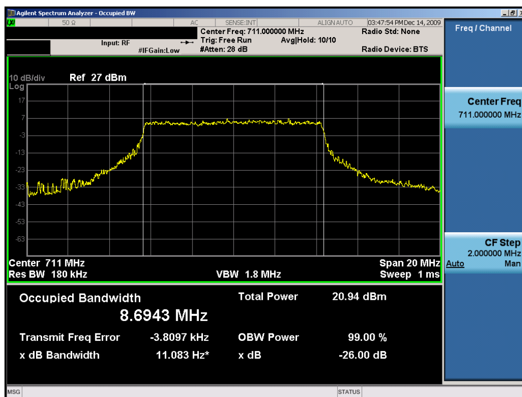
Plot 7-18. Occupied Bandwidth Plot (16-QAM Modulation – 711MHz)
