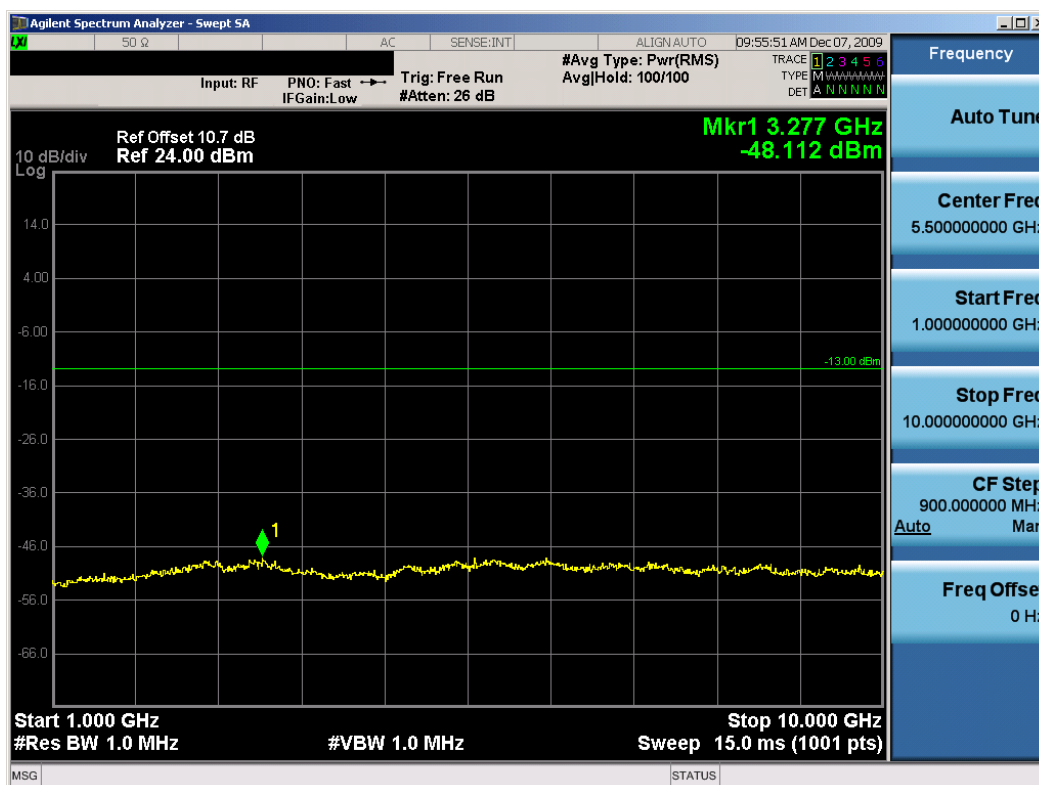
Plot 7-10. Conducted Spurious Plot (QPSK Modulation – 709MHz)
