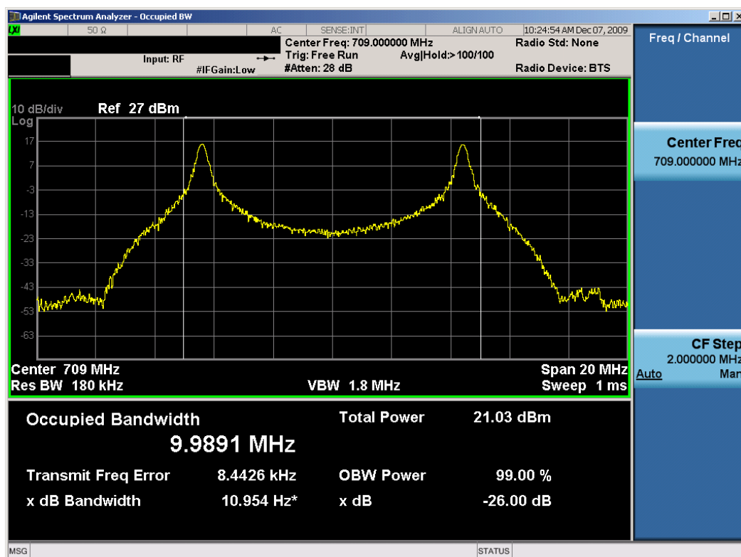
Plot 7-4. Occupied Bandwidth Plot (BPSK Modulation – 709MHz)
