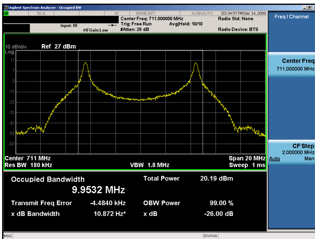
Plot 7-16. Occupied Bandwidth Plot (BPSK Modulation – 711MHz)
