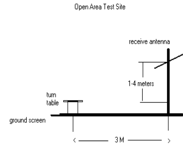
Figure 3-1. Diagram of 3-meter outdoor test range
