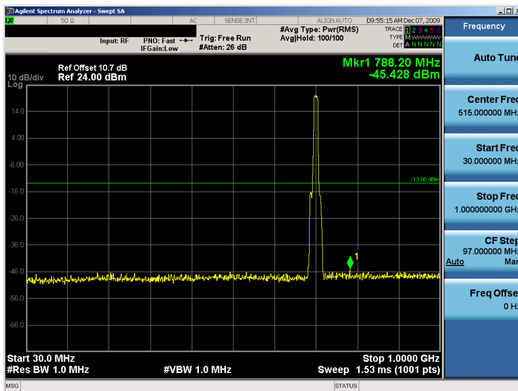
Plot 7-9. Conducted Spurious Plot (QPSK Modulation – 709MHz)
