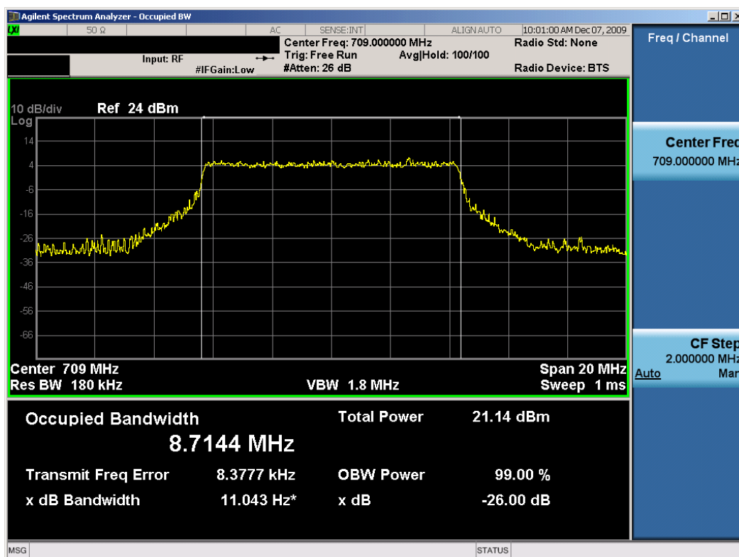
Plot 7-6. Occupied Bandwidth Plot (16-QAM Modulation – 709MHz)
