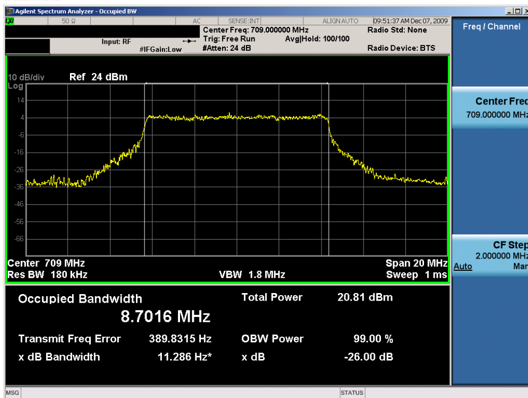
Plot 7-5. Occupied Bandwidth Plot (QPSK Modulation – 709MHz)
