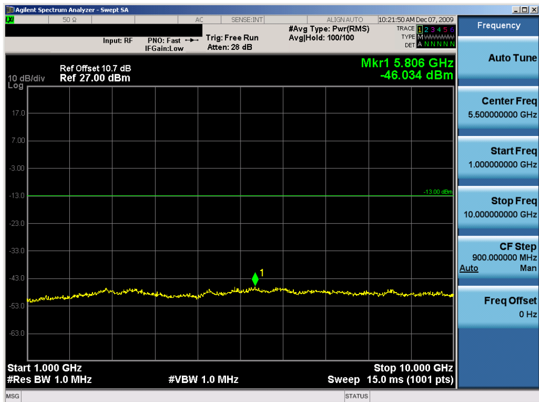
Plot 7-8. Conducted Spurious Plot (BPSK Modulation – 709MHz)
