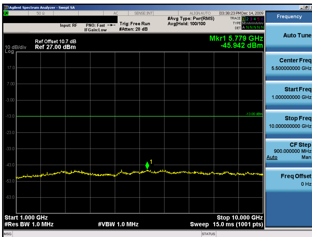
Plot 7-20. Conducted Spurious Plot (BPSK Modulation – 711MHz)
