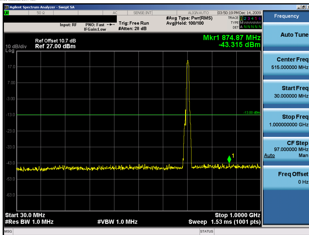
Plot 7-23. Conducted Spurious Plot (16-QAM Modulation – 711MHz)
