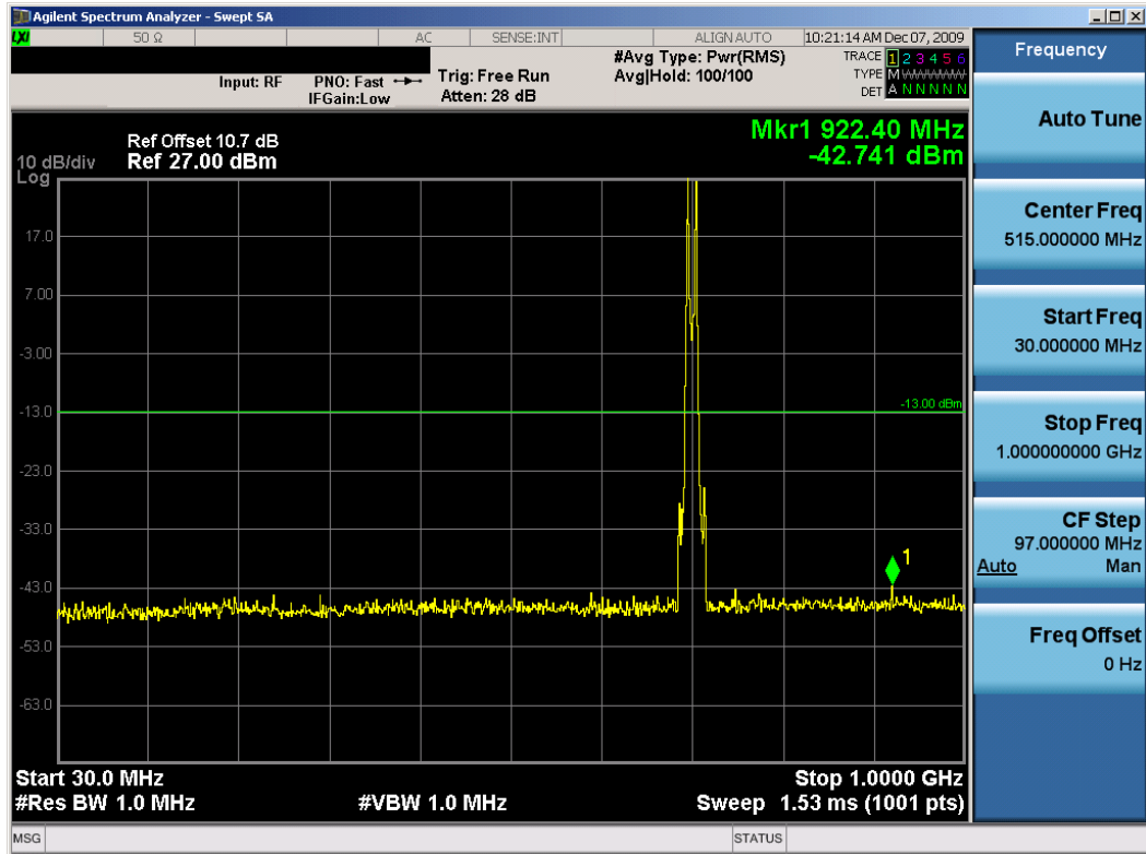
Plot 7-7. Conducted Spurious Plot (BPSK Modulation – 709MHz)
