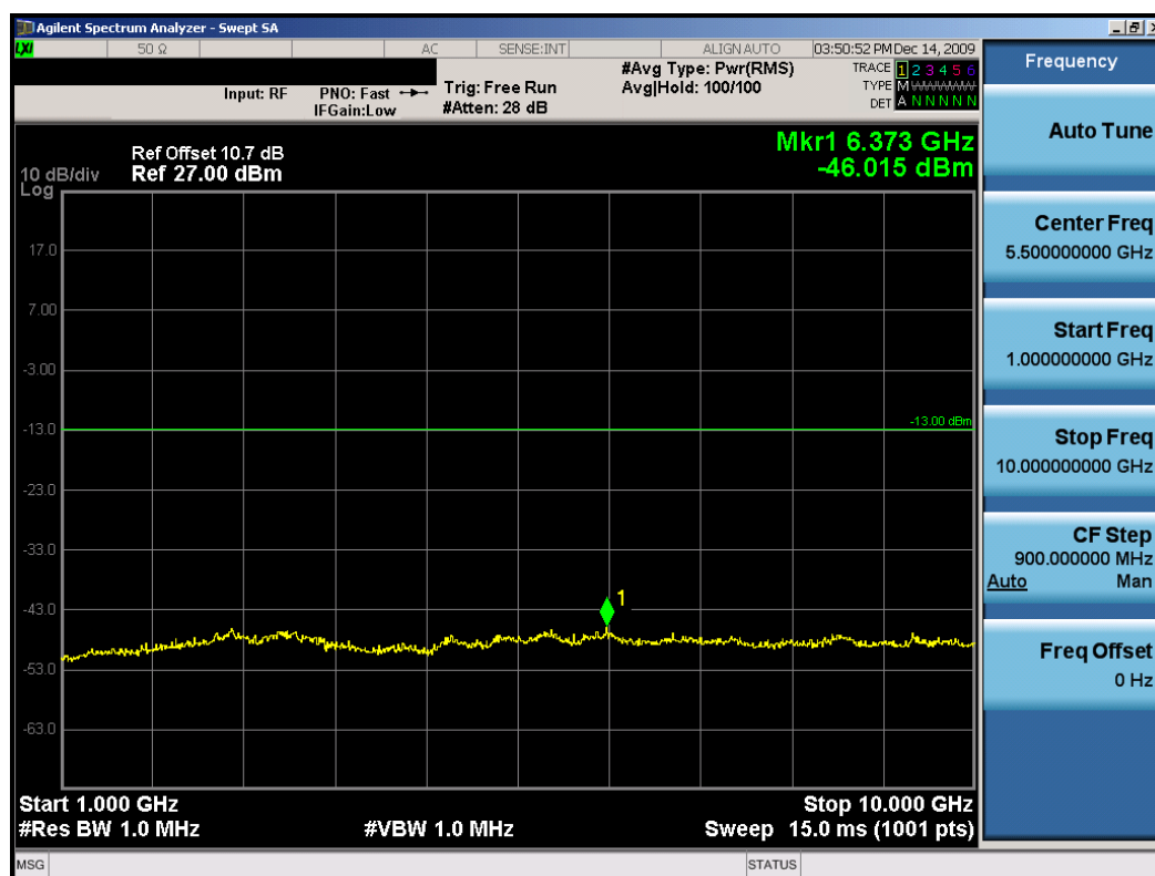
Plot 7-24. Conducted Spurious Plot (16-QAM Modulation – 711MHz)
