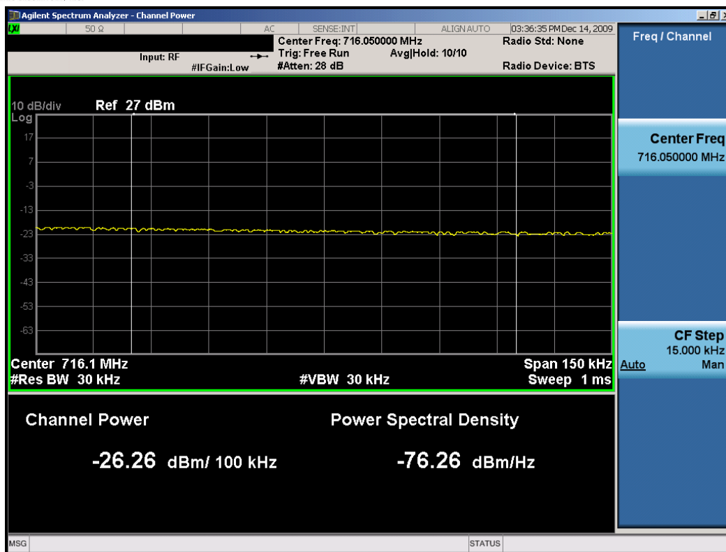
Plot 7-13. Band Edge Plot (BPSK Modulation – 711MHz)
