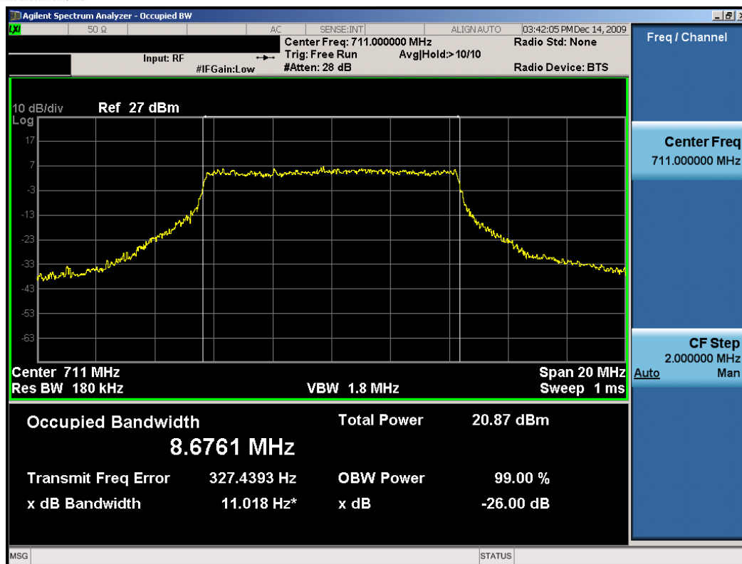
Plot 7-17. Occupied Bandwidth Plot (QPSK Modulation – 711MHz)
