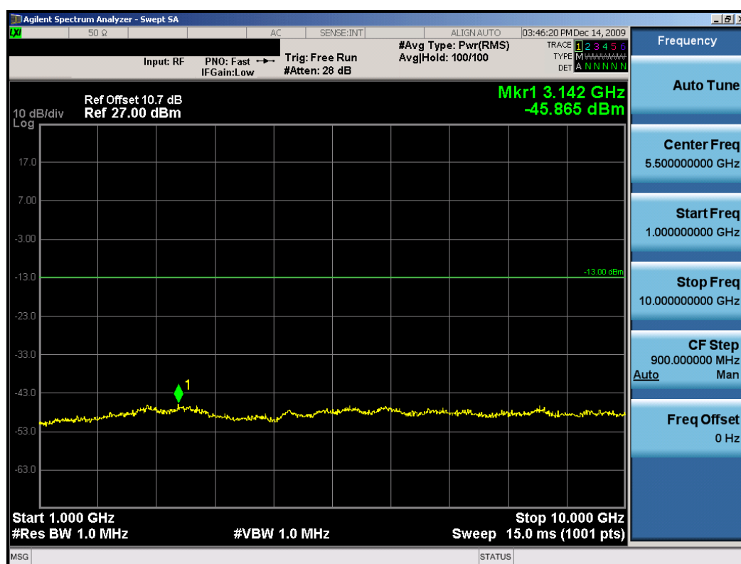
Plot 7-22. Conducted Spurious Plot (QPSK Modulation – 711MHz)
