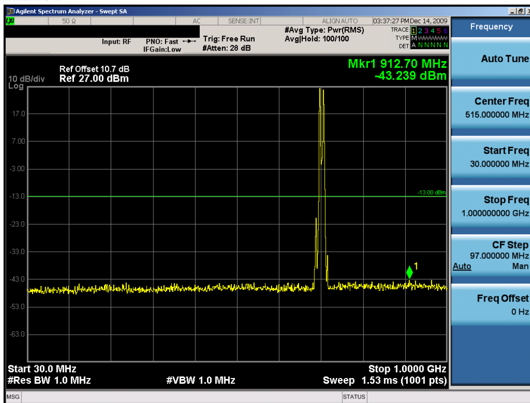
Plot 7-19. Conducted Spurious Plot (BPSK Modulation – 711MHz)
