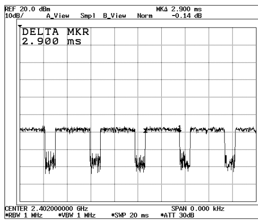
CH 00 2402MHz
