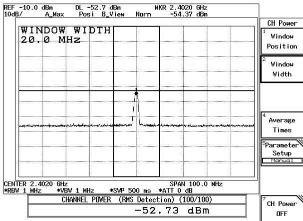
Channel 00
