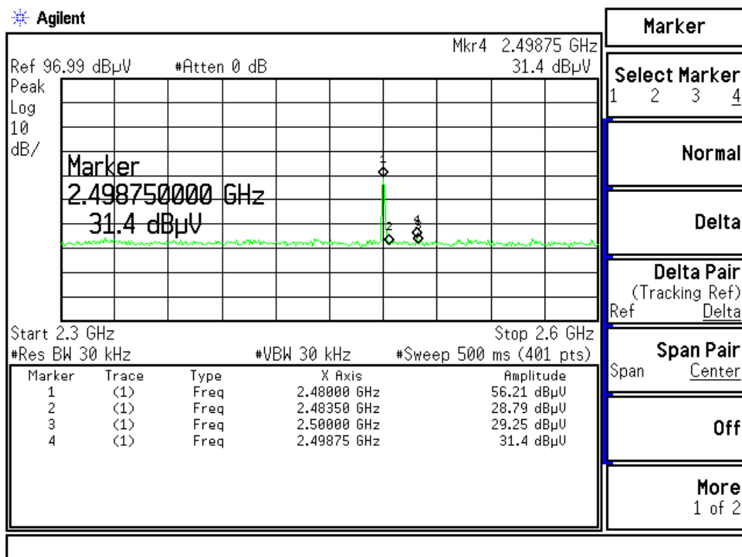
Figure Channel 78: (Vertical)
