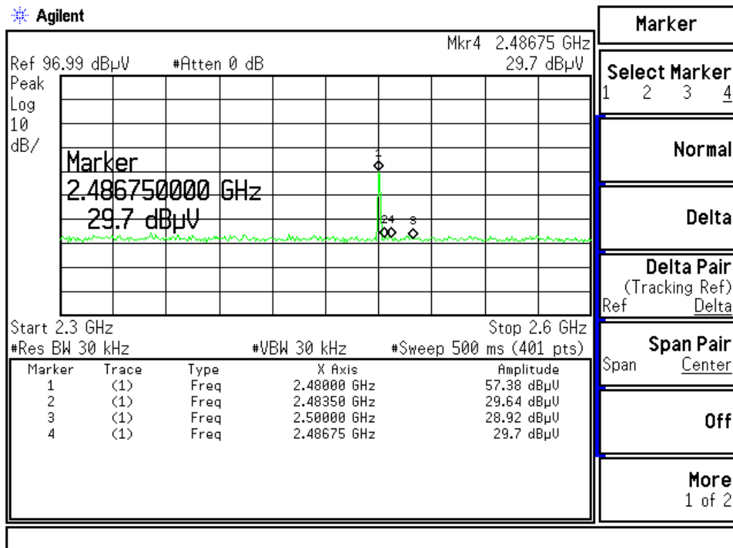
Figure Channel 78: (Horizontal)
