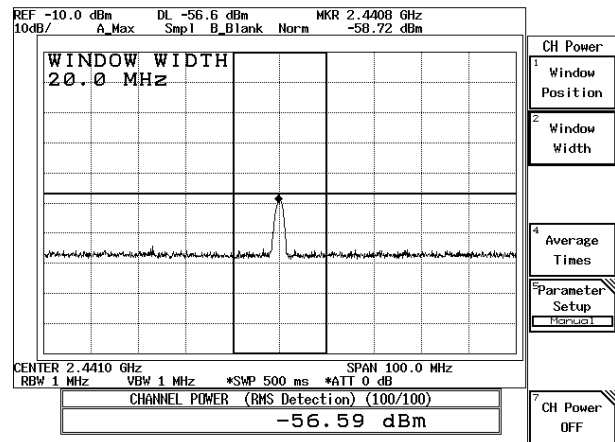
Channel 39
