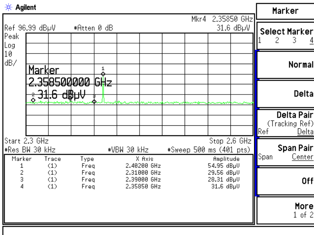
Figure Channel 00: (Vertical)
