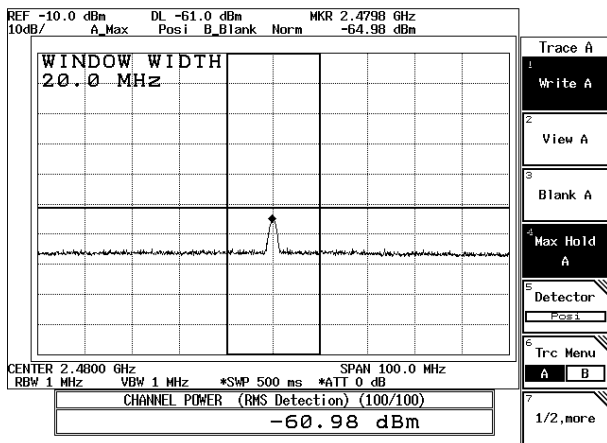
Channel 78
