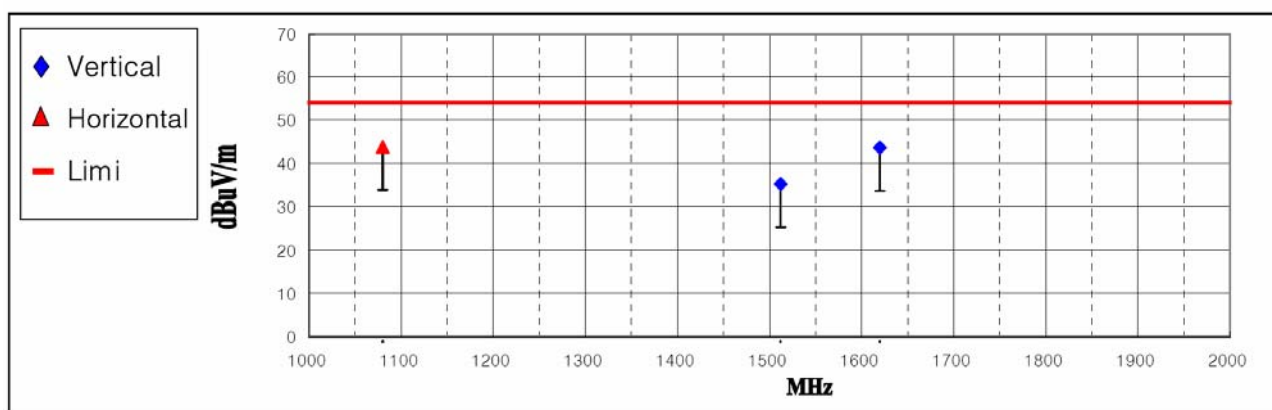
< Fig 7. Radiated Emission result (1000MHz ~ 2000MHz) >
