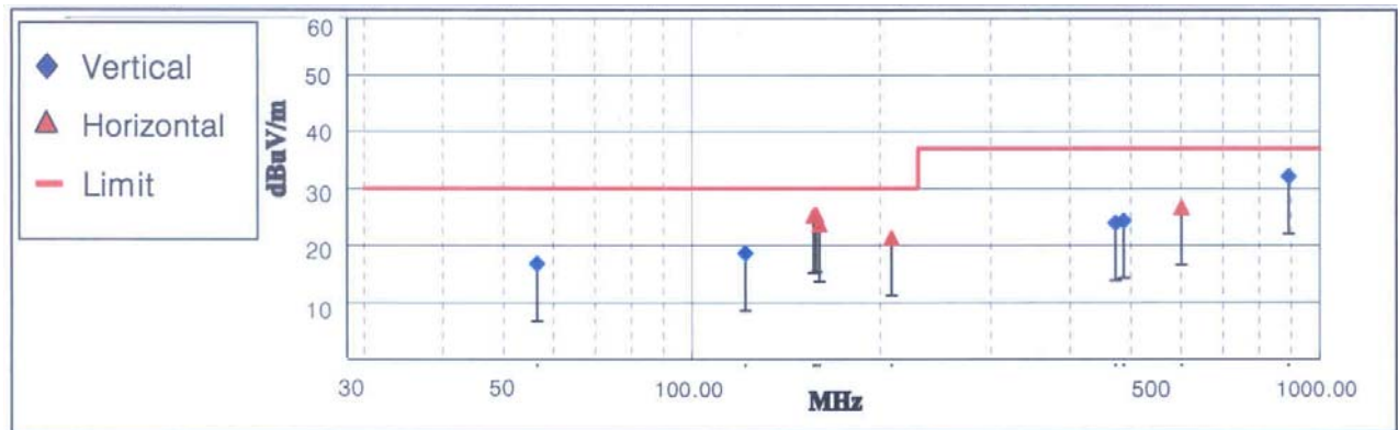
< Fig 6. Radiated Emission _ Digital (30MHz ~ 1000MHz) >
