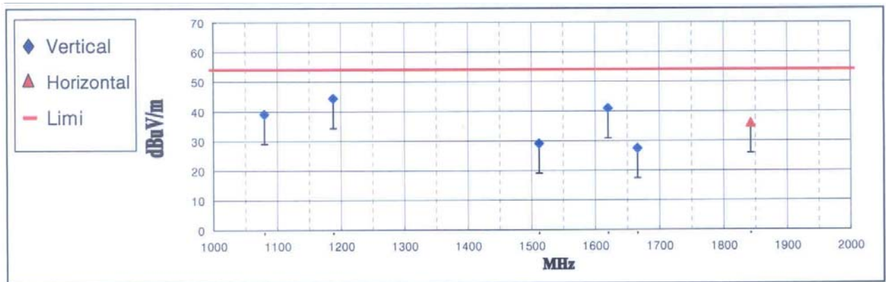
< Fig 7. Radiated Emission _ Digital (1000MHz ~ 2000MHz) >
