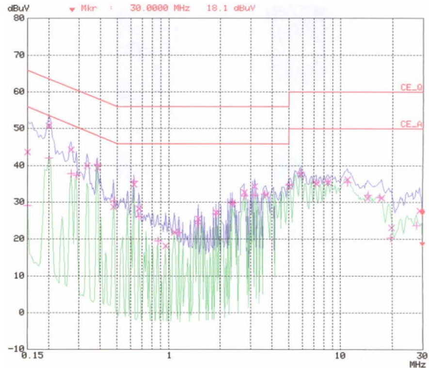
< Neutral line >
