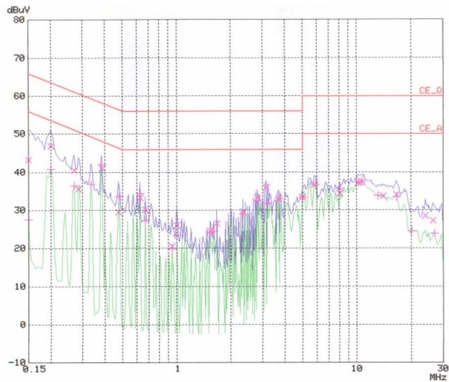
< Hot line >
