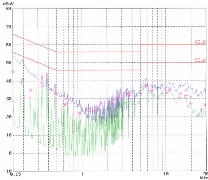
< Neutral line >
