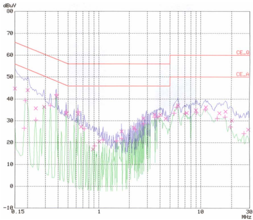
< Hot line >
