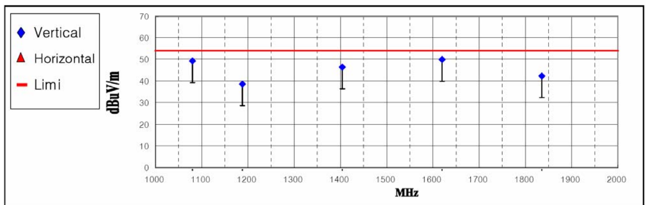
< Fig 5. Radiated emission result (1000MHz ~ 2000MHz)>
