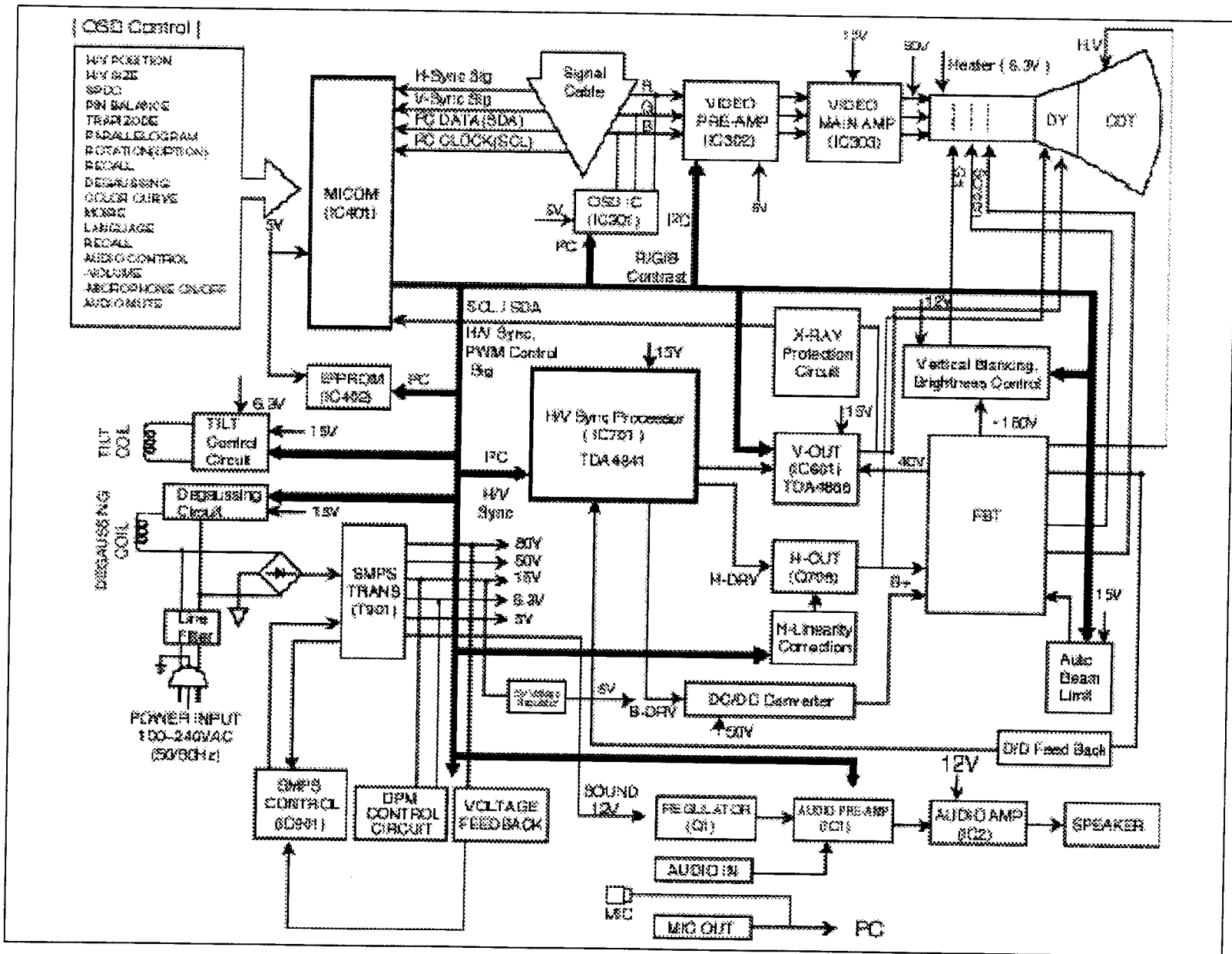
BLOCK DIAGRAM
