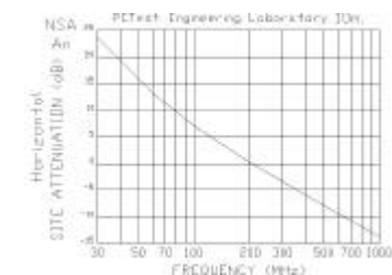
Fig. 5. NSA Theoretical Attenuation Curves (Horiz. Pol.)
