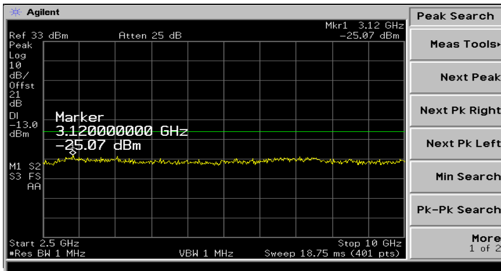
PLOTS OF EMISSION (GSM): Out of Band(Ch251)
