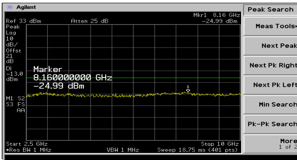
PLOTS OF EMISSION (EDGE): Out of Band(Ch251)
