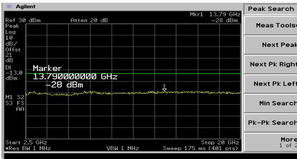
PLOTS OF EMISSION (EDGE): Out of Band(Ch810)
