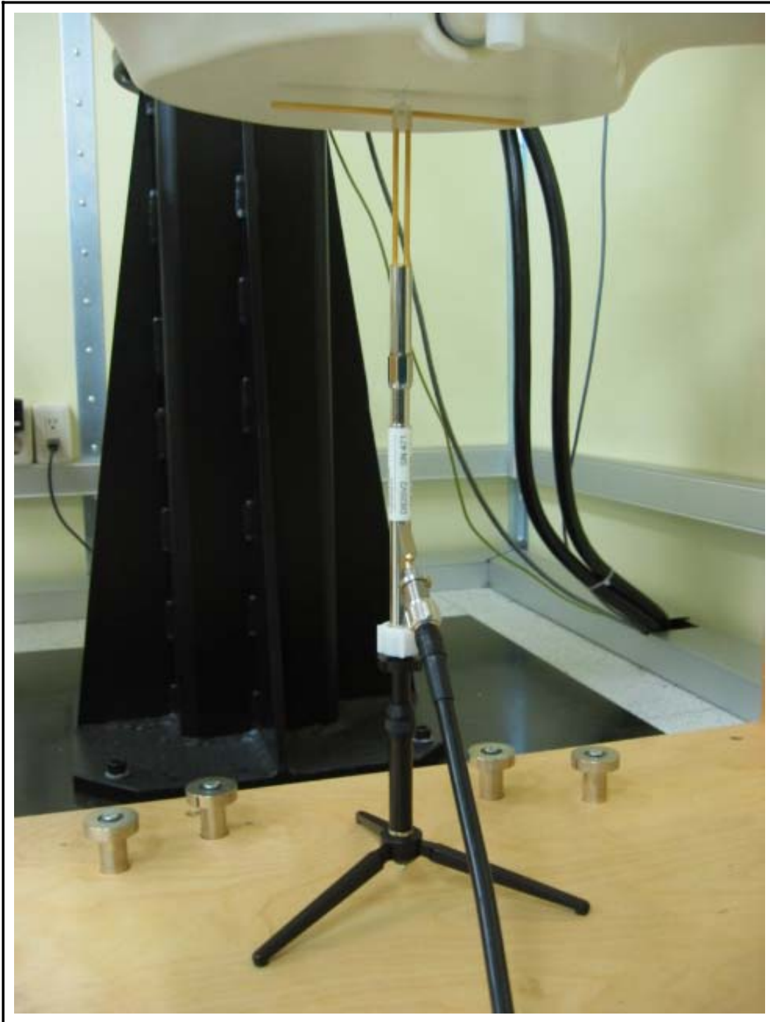
Figure 1 835 MHz Dipole Validation Test Setup
