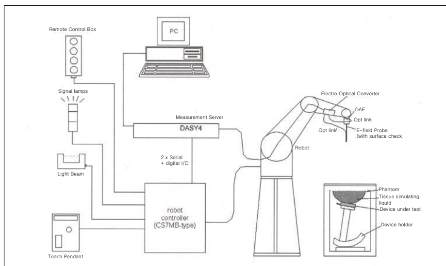
Figure 4.1 SAR Measurement System Setup
