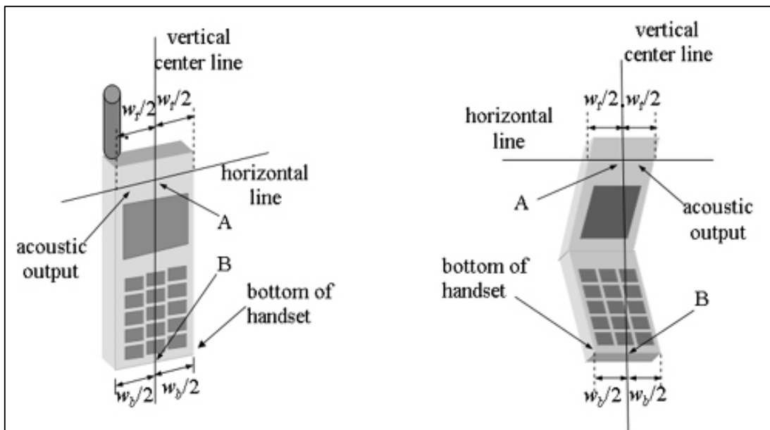
Figure 6.4 Handset Vertical Center & Horizontal Line Reference Points
