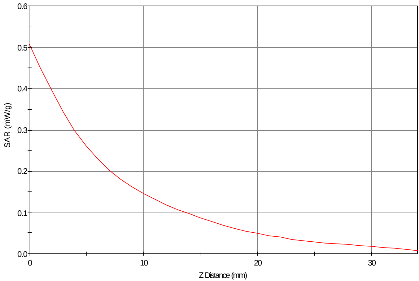
SAR - Z Axis at Hotspot x:-6.0 y:10.0
