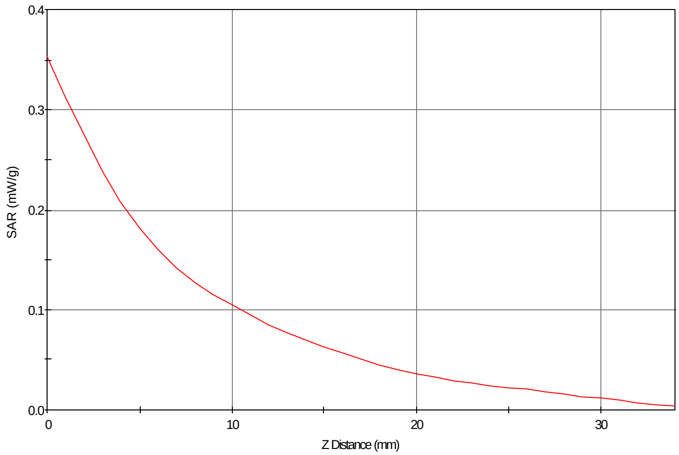
SAR - Z Axis at Hotspot x:-1.0 y:9.0
