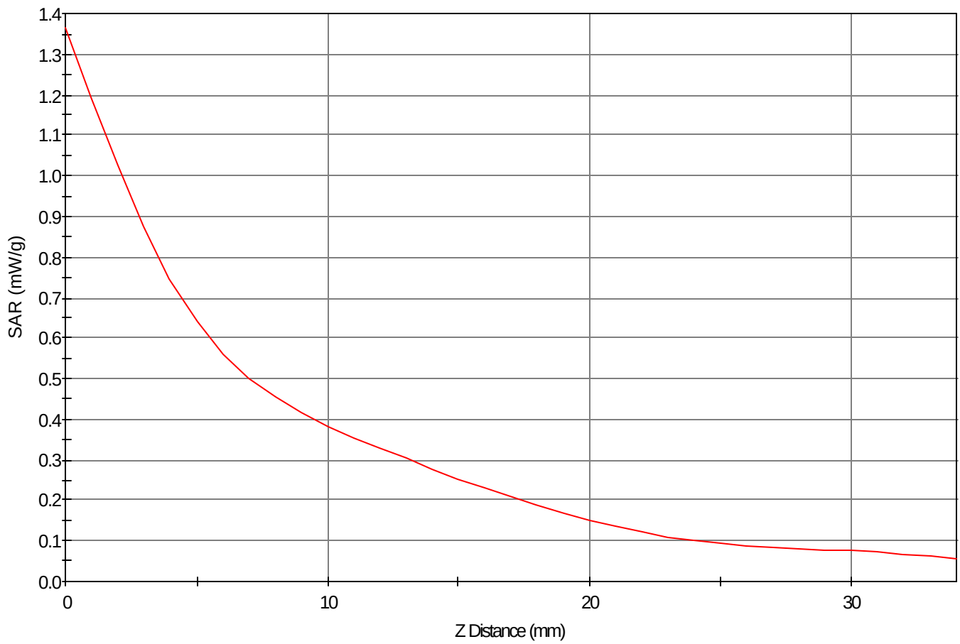
SAR - Z Axis at Hotspot x:6.0 y:-19.0
