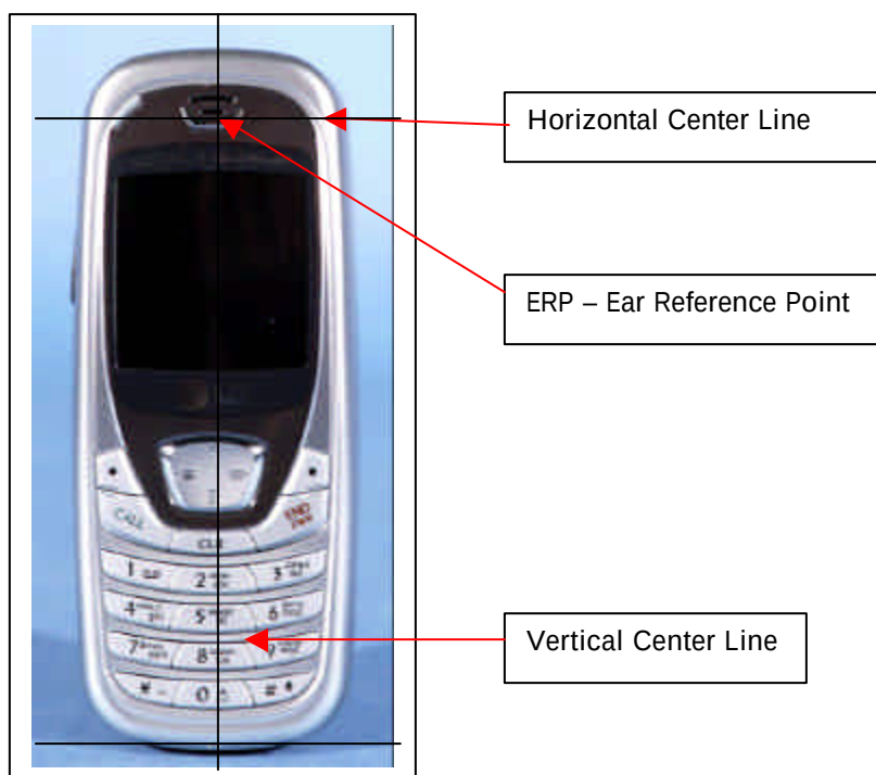
Figure 12.1 Handset Reference Points
