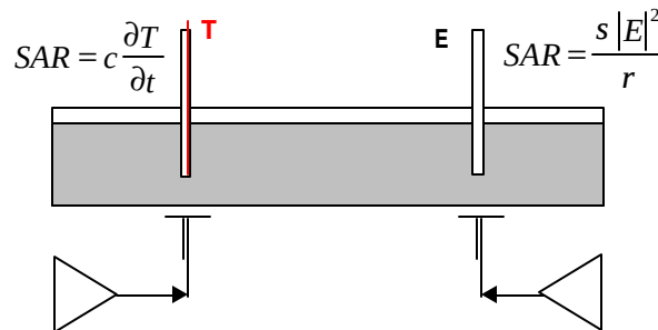
Figure 4.1 Temperature Assessment Test Configuration
