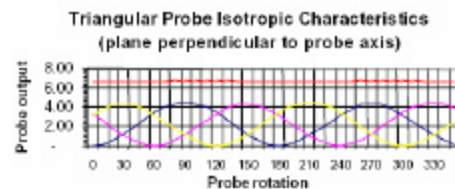
Figure 3.3 Probe Characteristics
