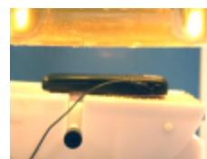
Figure A.9 Body SAR Test Setup -- w/o Belt Clip --
