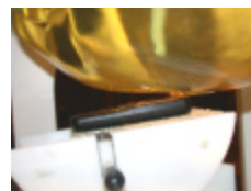
Figure A.4 Left Head SAR Test Setup -- Ear / 15° Tilt Position --
