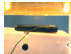
Figure A.10 Body SAR Test Setup -- w/o Belt Clip --
