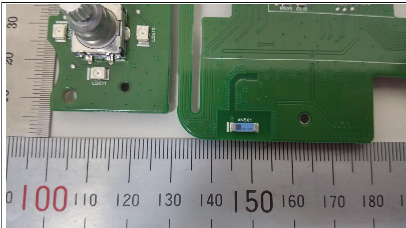
<BT Antenna>
