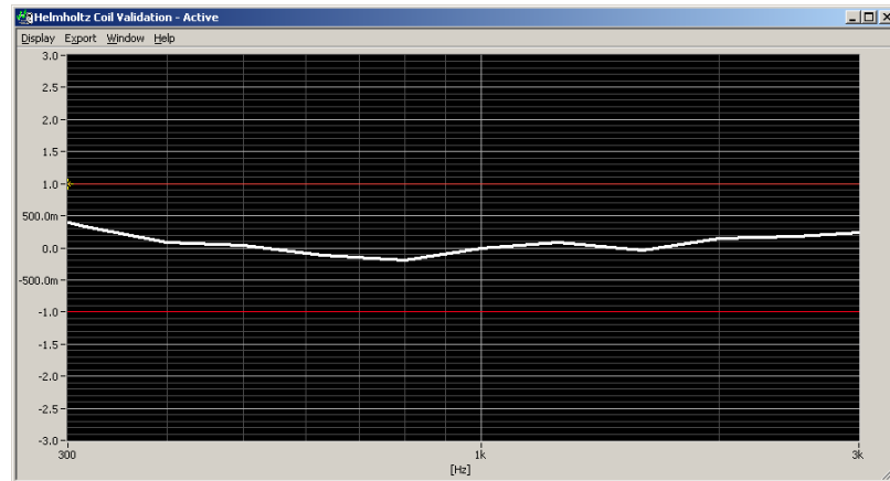
Figure 6-3 Helmholtz Coil Validation for Frequency Response
