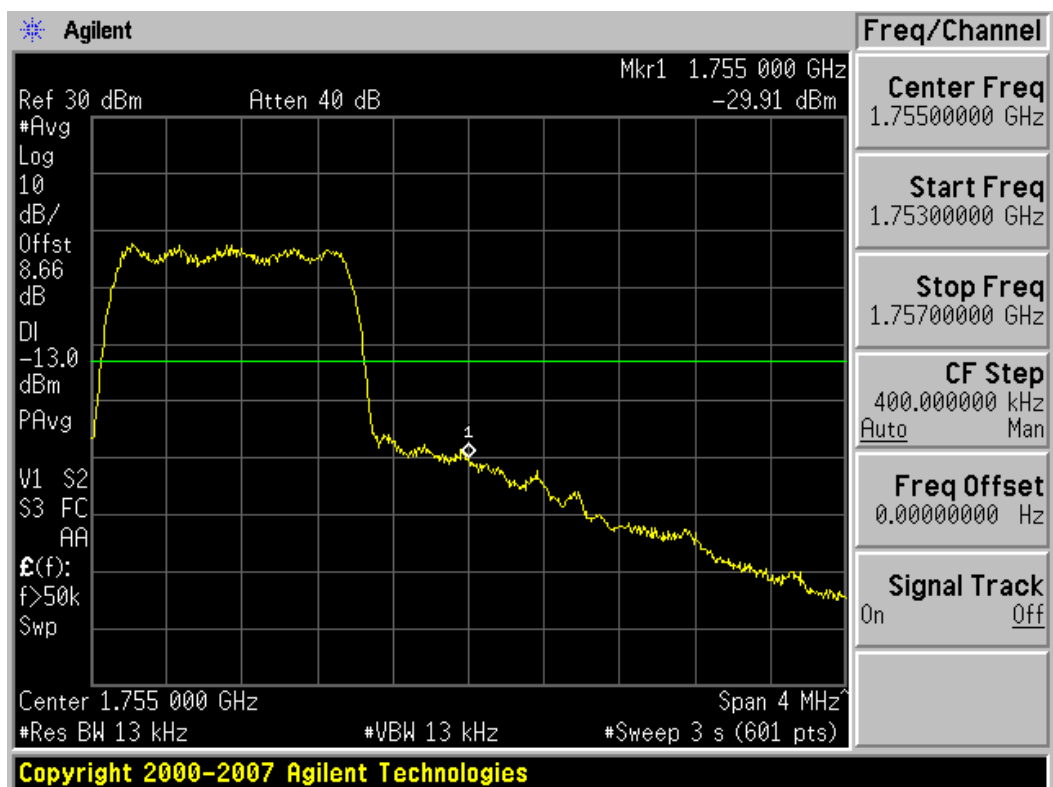
Plot 7-22. Band Edge Plot (AWS CDMA Mode – Ch. 875)
