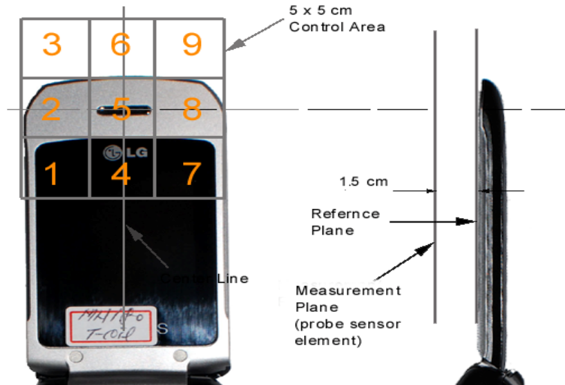
Figure 17-3 5x5 Scan grid above WD
