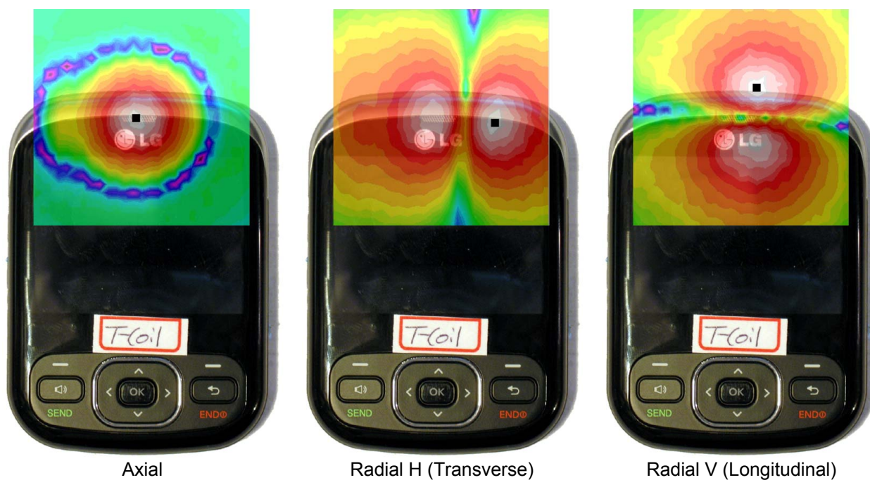
Figure 13-3 T-Coil Scan Overlay Magnetic Field Distributions
