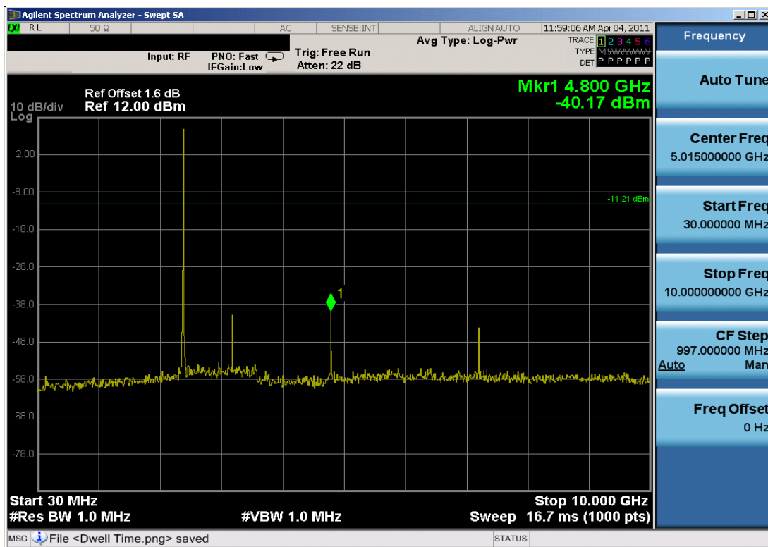
Plot 6-18. Conducted Spurious Plot (Bluetooth, 3Mbps – Ch. 0)
