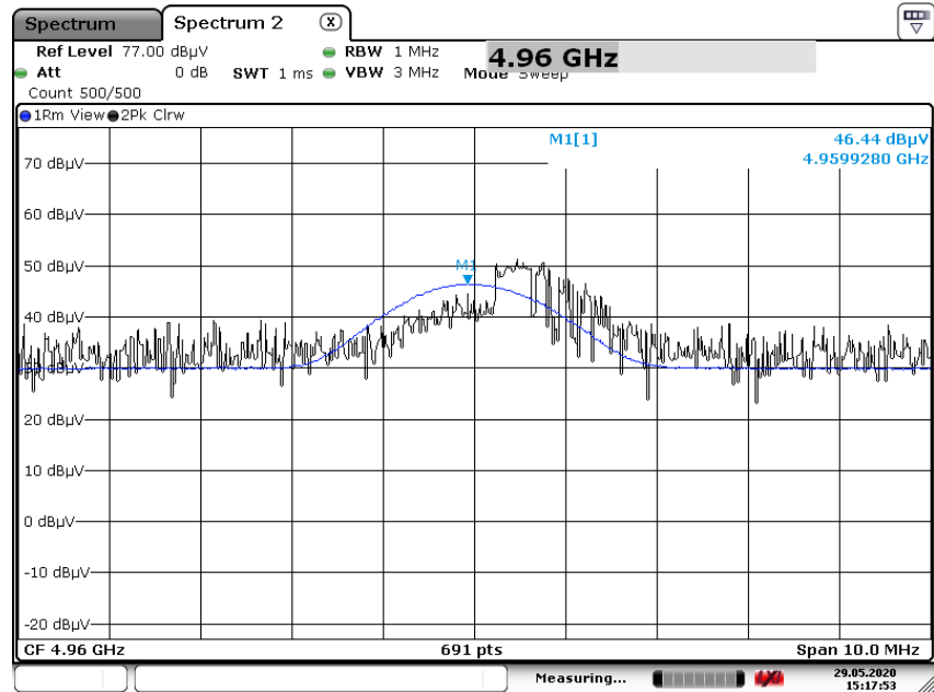
Radiated Spurious Emissions plot – Average Reading (Ch.39 2nd Harmonic)
