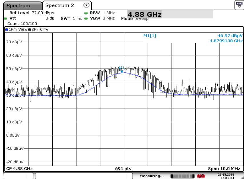
Radiated Spurious Emissions plot – Average Reading (Ch.19 2nd Harmonic)
