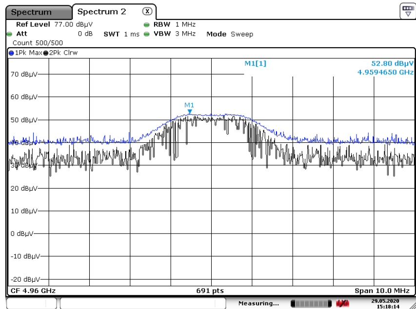
Radiated Spurious Emissions plot – Peak Reading (Ch.39 2nd Harmonic)
