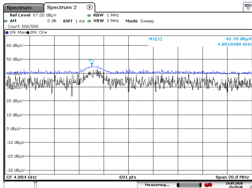
[Rx Worst case test plot_Peak Reading_Ch.0_X-H]
