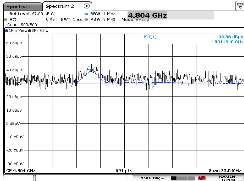
[Rx Worst case test plot_Average Reading_Ch.0_X-H]
