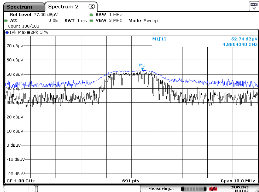
Radiated Spurious Emissions plot – Peak Reading (Ch.19 2nd Harmonic)
