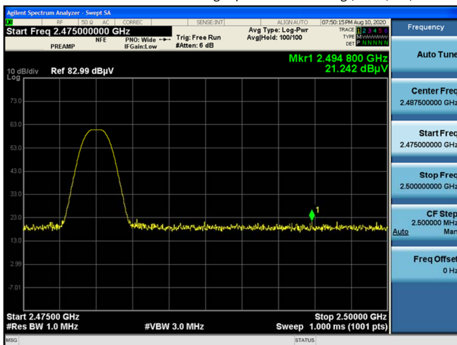
Radiated Restricted Band Edges plot – Peak Reading (Ch.39, Y-V)
