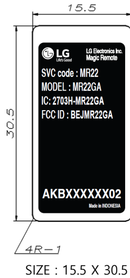
MR21GA Label size
