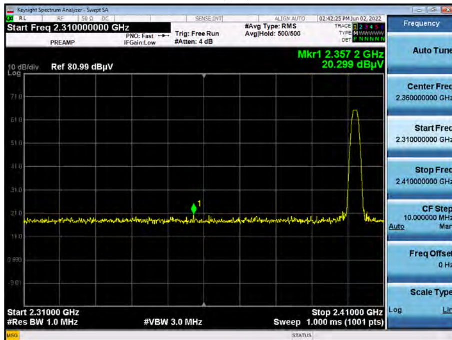
Radiated Restricted Band Edges plot – Peak Result (Ch.0, H)
