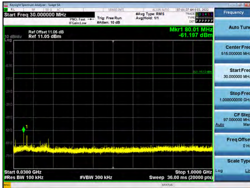
Conducted Spurious Emission (Mid-CH 16)
