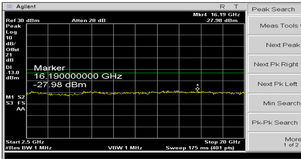
PLOTS OF EMISSION (EDGE): Out of Band(Ch810)
