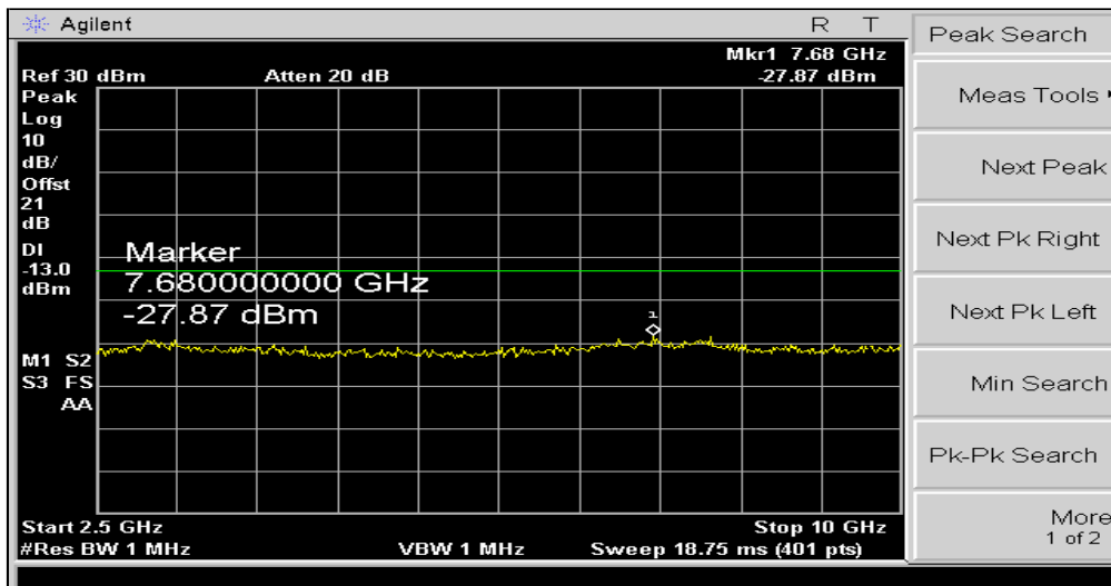
PLOTS OF EMISSION (EDGE): Out of Band(Ch251)
