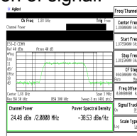
Figure 8-1 Signal Generator Modulated Signal
