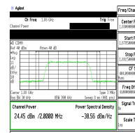
Figure 8-2 Wireless Device Modulated Signal
