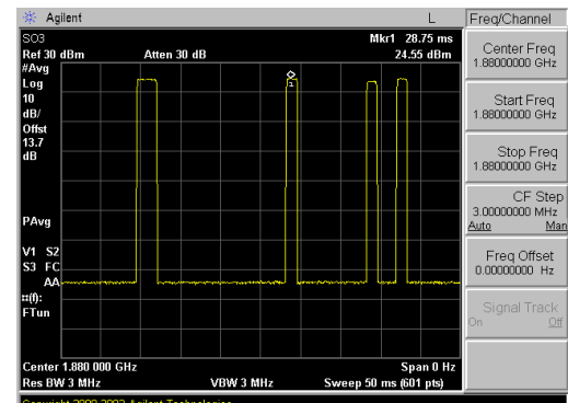
Figure 8-4 Zero-Span Plots
