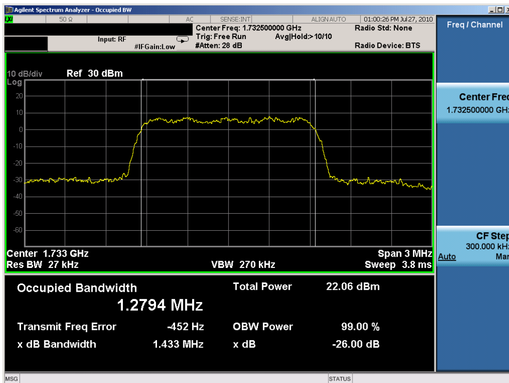
Plot 7-18. Occupied Bandwidth Plot (AWS CDMA A Mode – Ch. 450)
